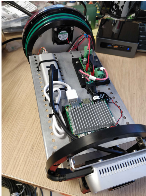
(A) Underwater Camera under development
