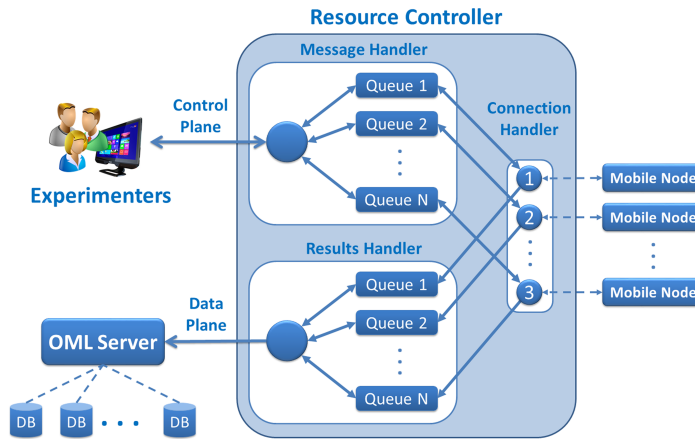
FIGURE 6.2: Resource Controller Architecture
