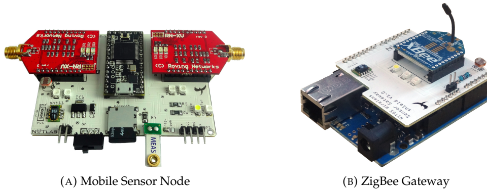
FIGURE 6.3: Custom-built Hardware of the NITOS BikesNet Platform
