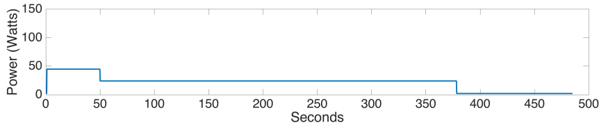
FIGURE 7.8: Simulated LAUV Motor Power Consumption
