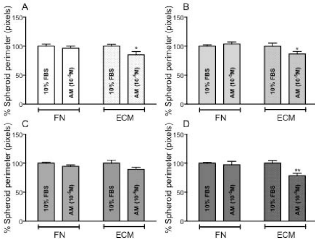
Figure 20: Mean \pm SEM % spheroid perimeter comparisons between control and amiloride treated cells. A , MeT-5A, B , M14K, C , MSTO-211H and D , ZL34. * indicates p < 0.05 and **, p < 0.01 . n = 12 .
