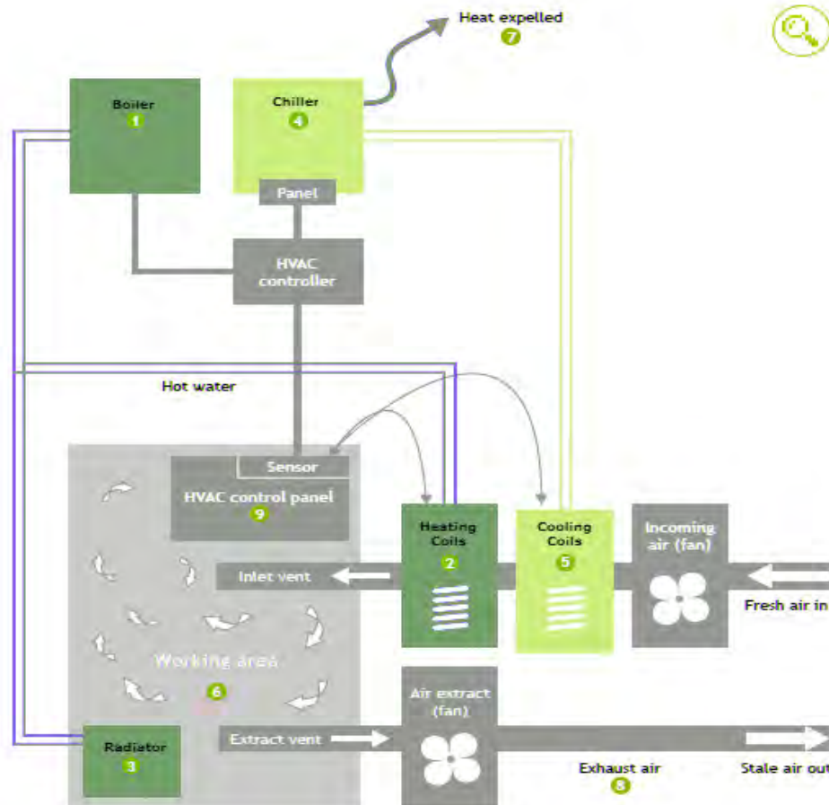
HVAC components [170]
