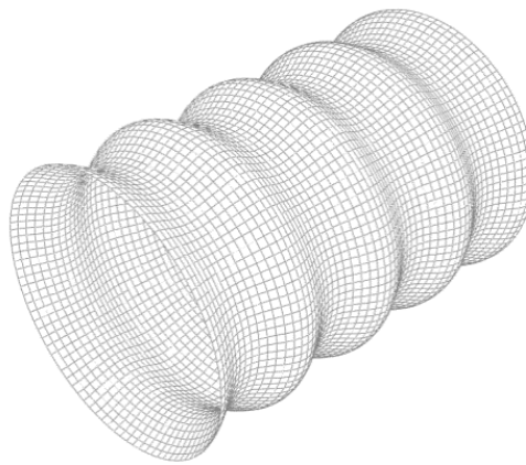
Figure 6 - 4: Bifurcation (first wrinkling) shape of axially loaded stainless steel cylinder ( D/t_s = 26.3 ).
