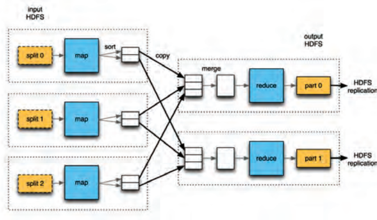
Figure 10.1: Overview of Map/Reduce and Hadoop (from [47]).
