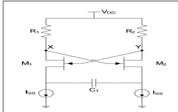
Figure 2.7 Relaxation Oscillator
