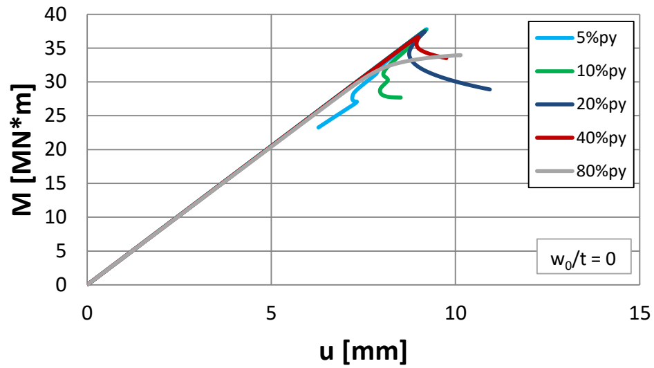
Figure 50: Base moment - displacement curves for e=5 and w_0/t = 0 .
