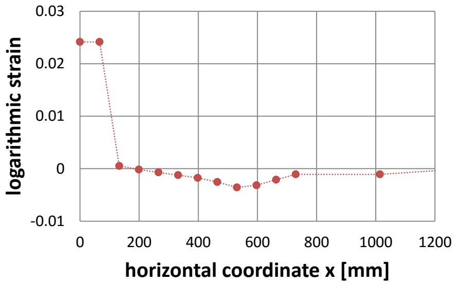
Figure 94: Logarithmic strain at the nodes of the tank base plate in terms of the horizontal coordinate x for Tank II, on the inner surface of the base plate at 0.119g.
