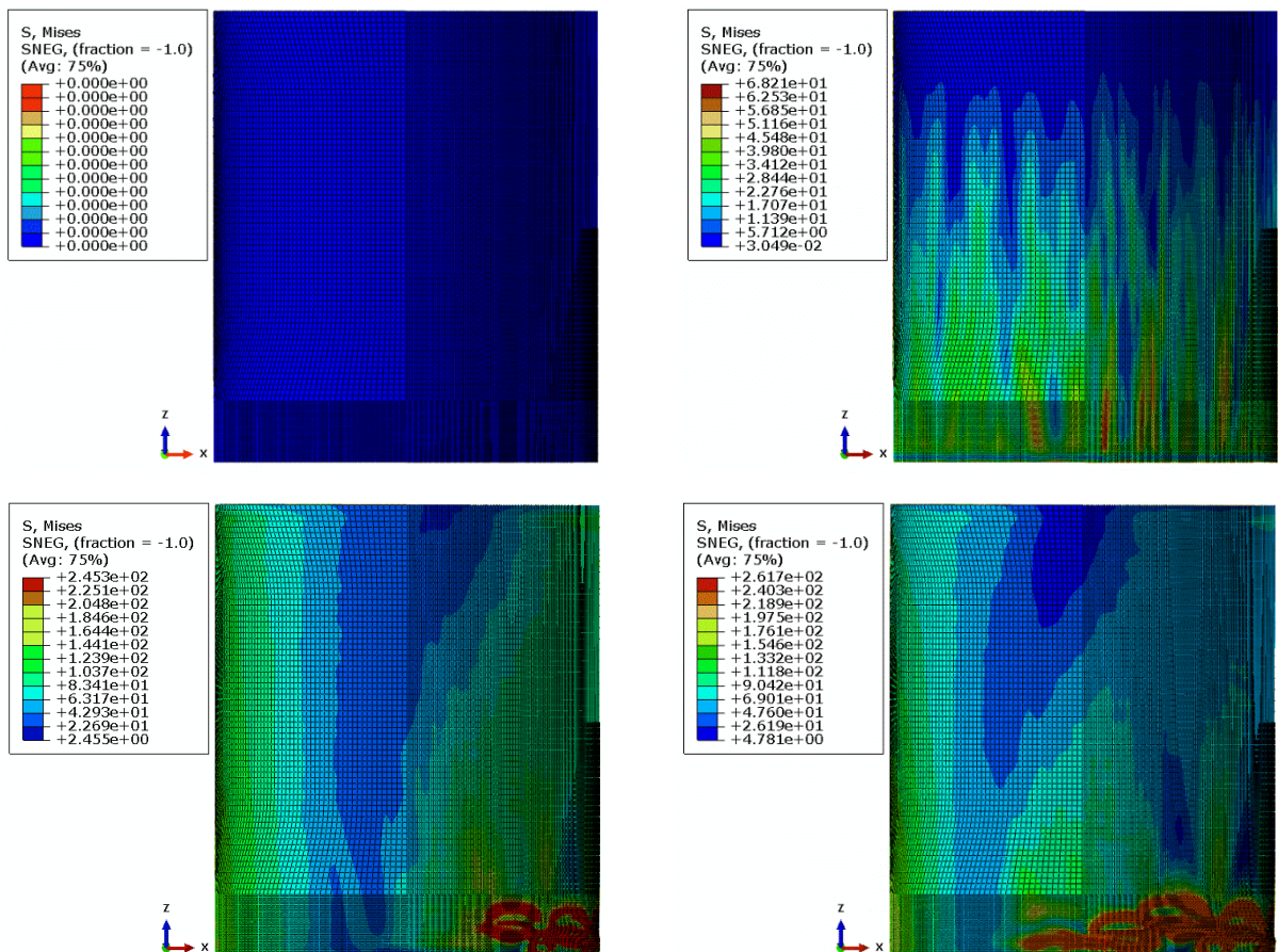
Figure 38: Consecutive stages of buckling of the tank under consideration for imperfection shape #1, e = 5 and w_0 / t = 0.63 . The first stage corresponds to the undeformed state and the second stage to the end of the acting of the hydrostatic pressure.
