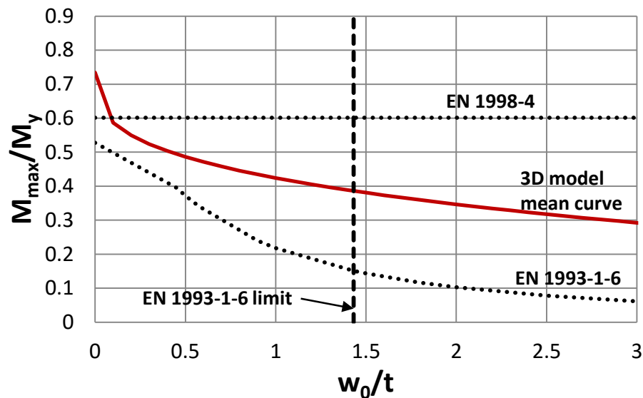
Figure 58: Normalized maximum moment in terms of imperfection for three-dimensional analysis and the relevant provisions of EN 1993-1-6 and EN 1998-4 in the case of hydrostatic pressure.
