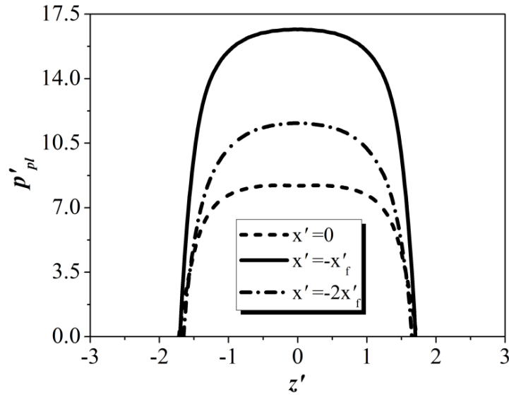
Figure 2-10: Dimensionless pressure distribution in the transverse direction ( z -direction) of a power-law fluid ( m=5 \times 10^4 \text{ Pa}\cdot\text{s}^n , n=0.35 ) for W_i/2H_o=80 with x'_f the dimensionless detachment point.
