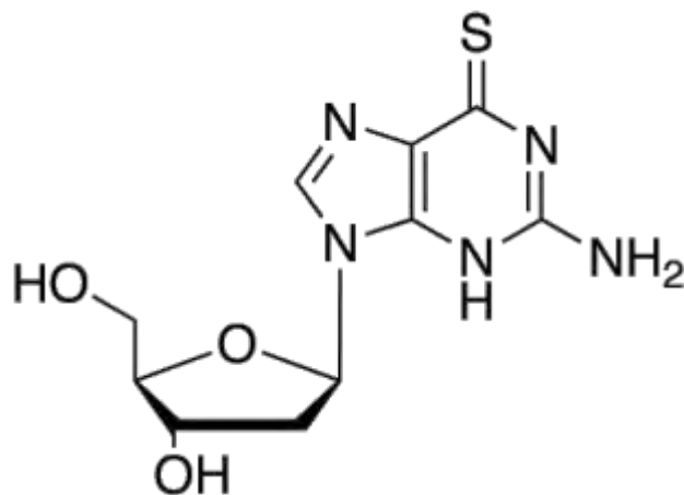
6-thioguanine
