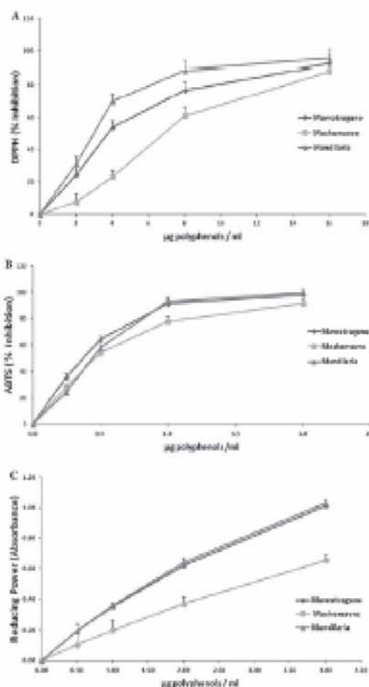
Figure 1. (A) Percentage 2,2-diphenyl-1-picrylhydrazyl (DPPH) radical scavenging activity, (B) percentage 2,2'-azino-bis(3-ethylbenzothiazoline-6-sulfonic acid) (ABTS) radical scavenging activity and (C) reducing power of grape stem extracts from Mavrotragano, Moshomavro and Mandilaria varieties. Values are presented as the means ± SEM.
