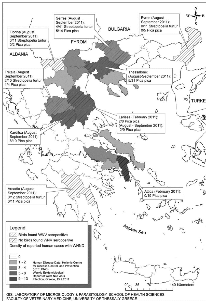
Figure 1. Occurrence of WNV human cases and results of serologic surveillance in wild magpies and turtle doves (Greece, February–September 2011). Map of Greece showing prefectures of Greece where occurrence of human cases of WNV was observed until 15 September 2011, in relevance to
