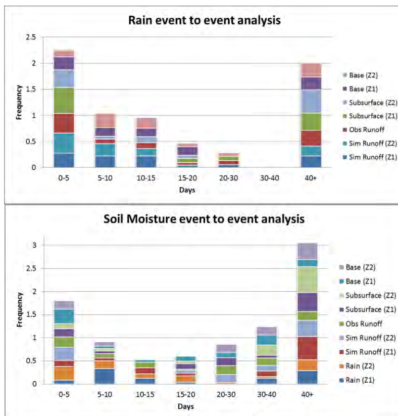
Figure 4.11: Semi-lumped model with 2 elevation zones, event to event analysis results for rain (top) and soil moisture (bottom) deficit time series. Z1 is the lowest elevation zone.
