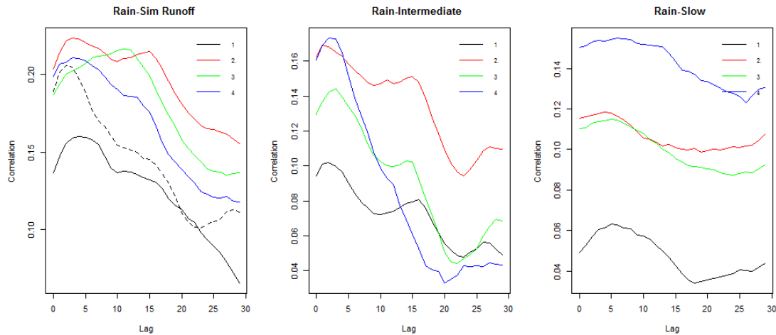
Figure 4.7: Four elevation zones semi-lumped model cross-correlation analysis for the rain deficit time series. Zone 1 always refers to the lowest elevation zone. The dashed line is the cross-correlation between the aggregated rain and observed runoff time series.
