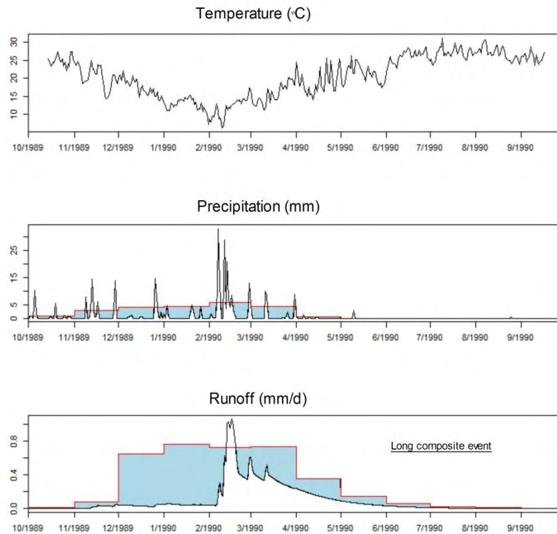
Figure 3.8: Example of composite drought event (1989-1990)
