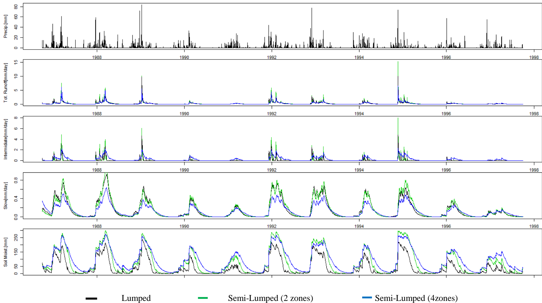
Figure 4.3: Comparison between the different simulations (lumped and semi-lumped with two and four elevation zones).
