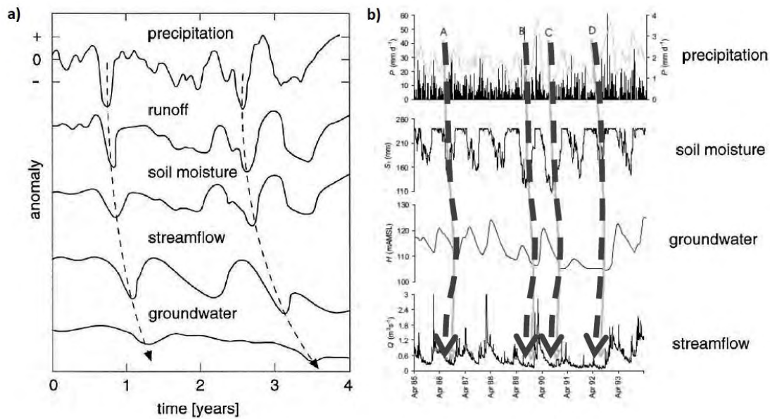
Figure 1.1: Propagation of a precipitation anomaly through the parts of the hydrological cycle for various variables (adapted from Van Loon, 2013), a) synthetic time series: 0 = mean, + = positive anomaly, - = negative anomaly [Changnon Jr, 1987], b) time series of the Pang catchment (UK): P = precipitation, Sr = soil moisture storage in the root zone, H = groundwater level, and Q = streamflow [Peters, 2003]. Propagation of drought events is indicated by the arrows.
