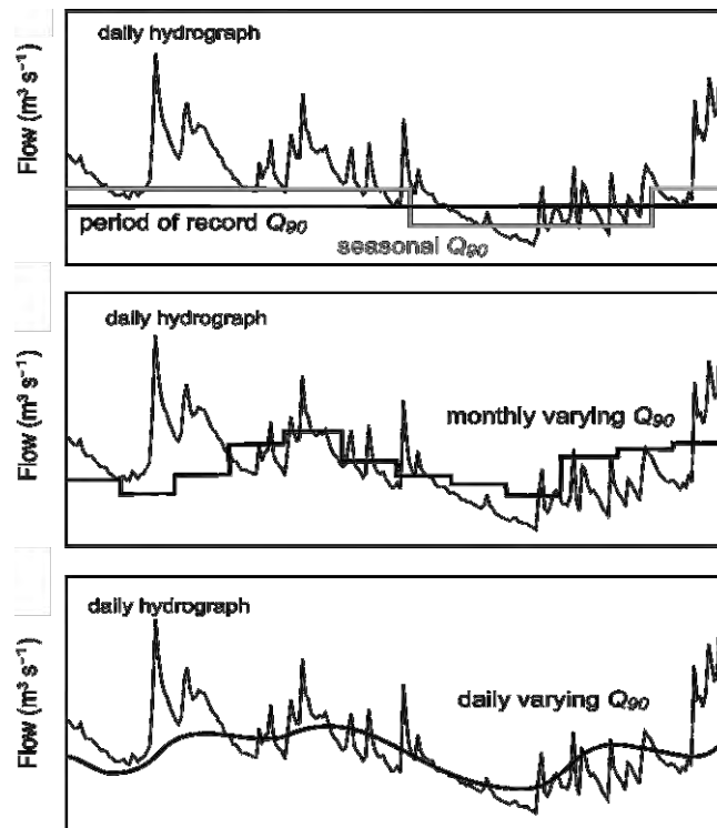
Figure 3.2: Illustration of threshold levels: fixed threshold (top); monthly varying threshold (middle); daily varying threshold (bottom) (adapted from WMO, 2008)
