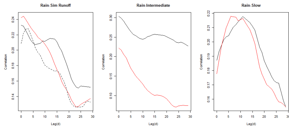
Figure 4.6: Two elevation zones semi-lumped model cross-correlation analysis for the rain deficit time series. Black line illustrates the lower zone and red line the higher elevation zone. The dashed line is the cross-correlation between the aggregated rain and observed runoff time series.
