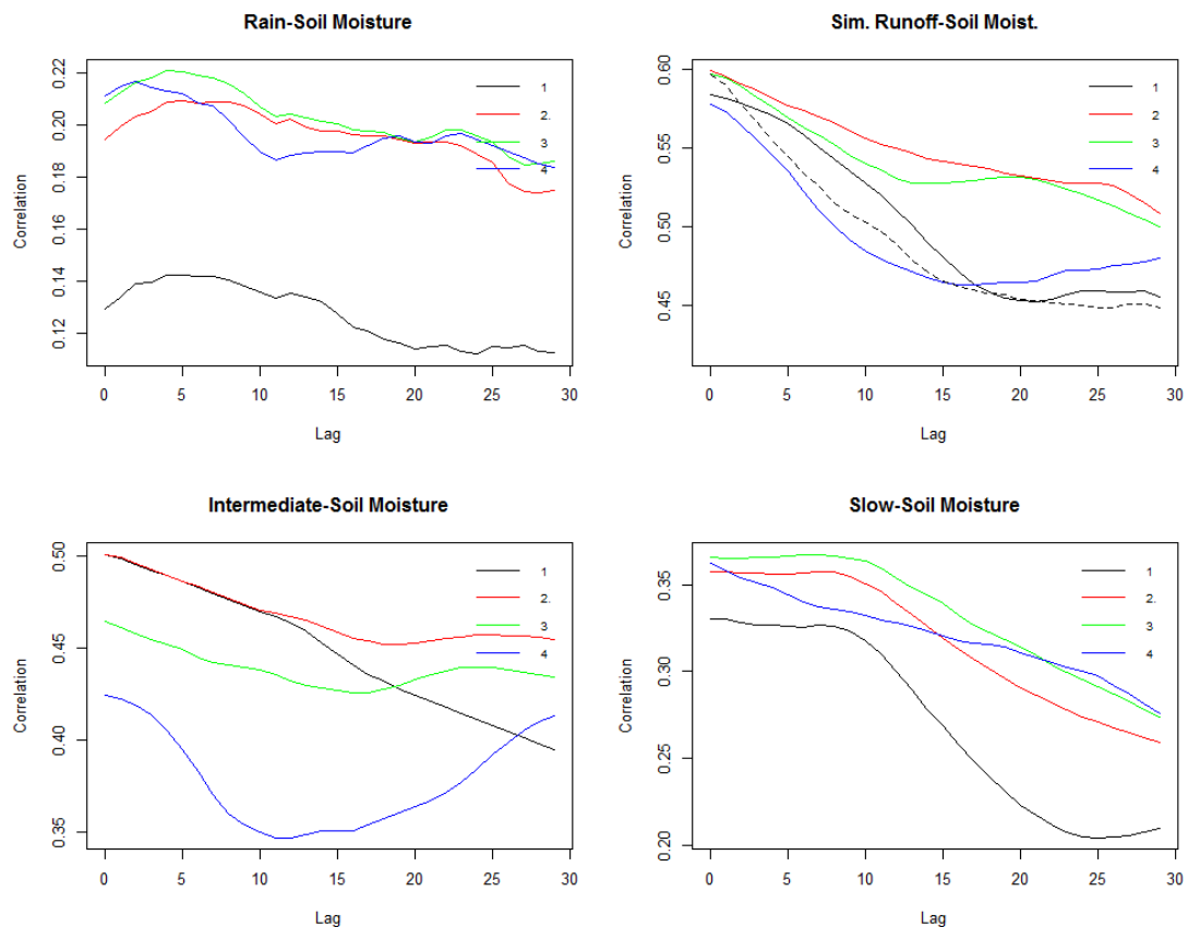
Figure 4.9: Four elevation zones semi-lumped model cross-correlation analysis for the soil moisture deficit time series. Zone 1 always refers to the lowest elevation zone. The dashed line is the cross-correlation between the aggregated soil moisture and observed runoff time series.
