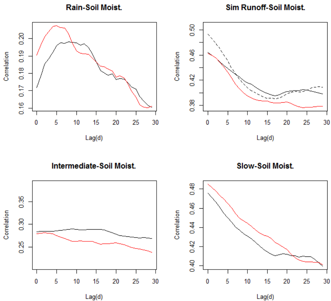
Figure 4.8: Two elevation zones semi-lumped model cross-correlation analysis for the soil moisture deficit time series. Black line illustrates the lowest zone and red line the highest elevation zone. The dashed line is the cross-correlation between the aggregated soil moisture and observed runoff time series.
