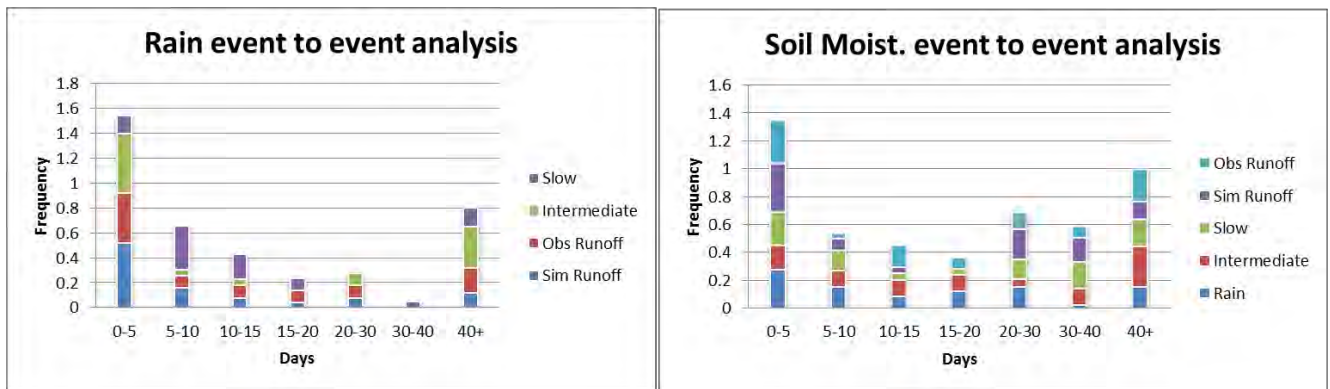
Figure 4.10: Lumped model event to event analysis results for rain (left) and soil moisture (right) deficit time series.
