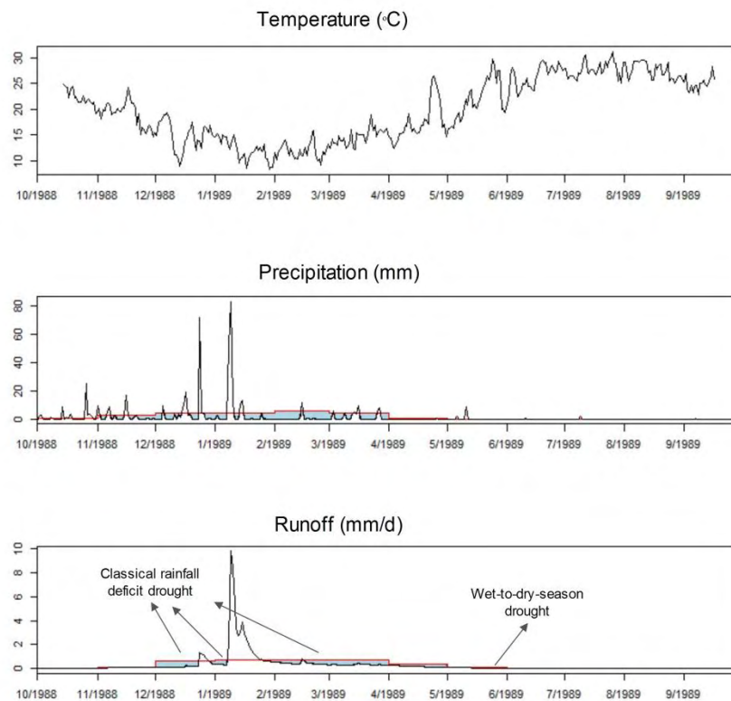
Figure 3.7: Example of classical rainfall deficit and wet-to-dry-season drought events (1988-1989)
