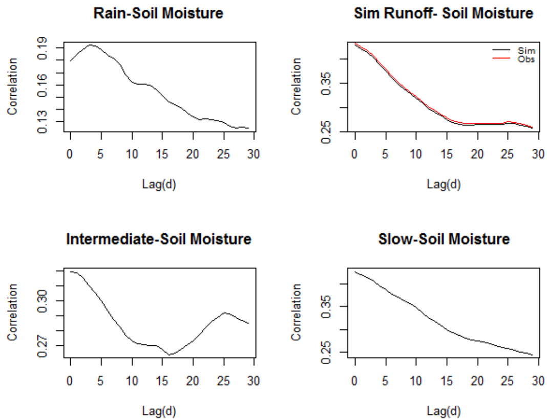
Figure 4.5: Cross-correlation analysis for the soil moisture deficit time series.
