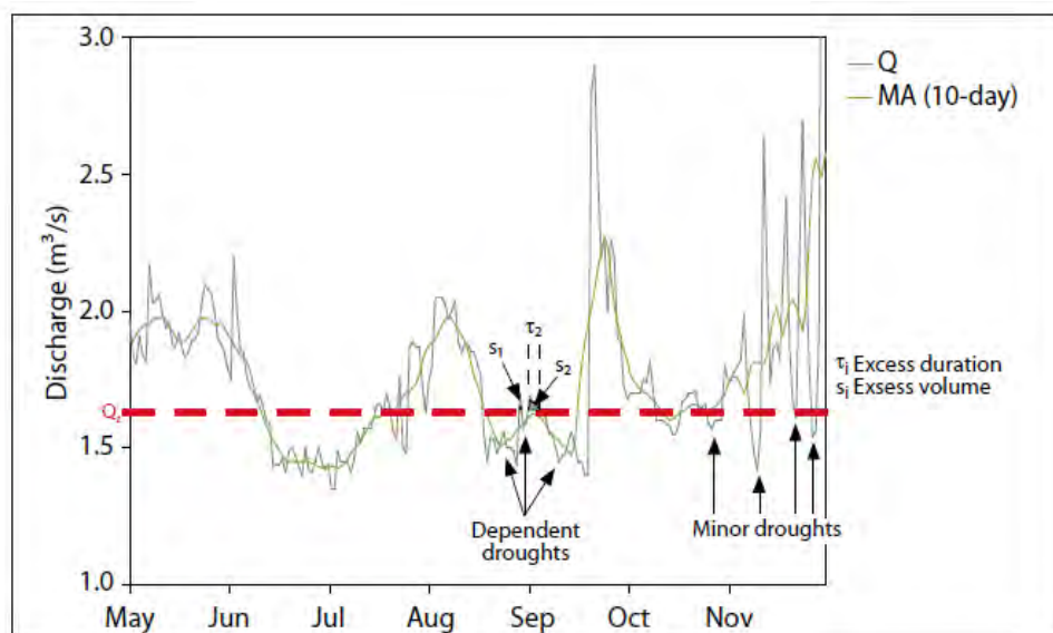
Figure 3.4: Illustration of pooling dependent deficits and removal of minor deficits by an MA(10-day) filter (adapted from WMO, 2008)
