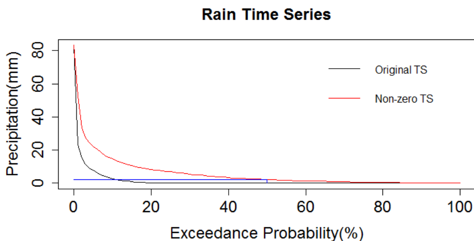
Figure 3.3: Flow duration curves for the original and non-zero rainfall time series. The Q_{50} of the non-zero time series corresponds to Q_{15} in the original time series.
