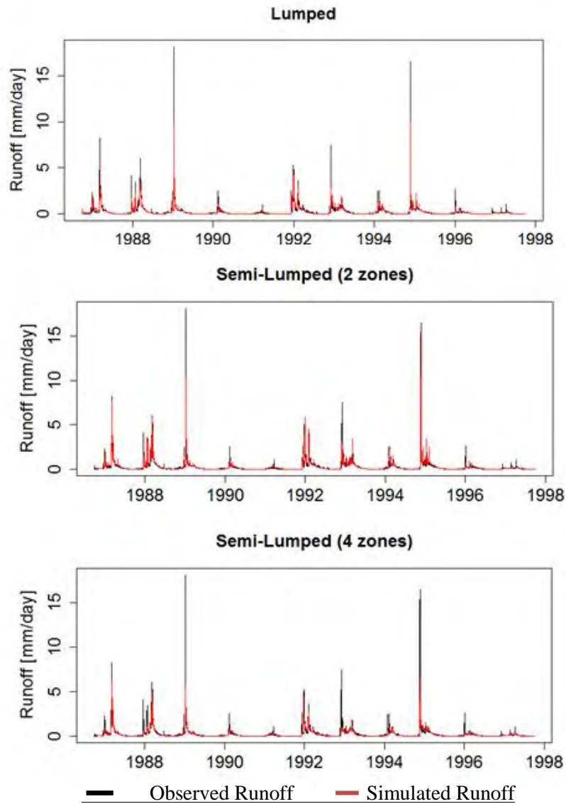
Figure 4.1: Observed and simulated runoff time series for the three different simulations. The plots correspond to the whole record of time series
