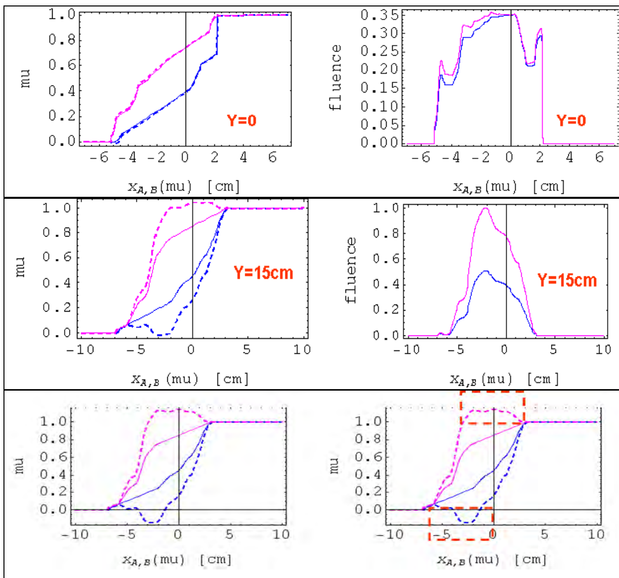
Figure 24: Different MLC corrections for different points from the center of the field, at the center ( upper ), for y=15\text{ cm} ( middle ) and for points >20\text{ cm} ( lower ). Y axis in these plots shows the MU delivered ( \mu ) while x axis represent the spatial distance x between two opposite leaves A, B.
