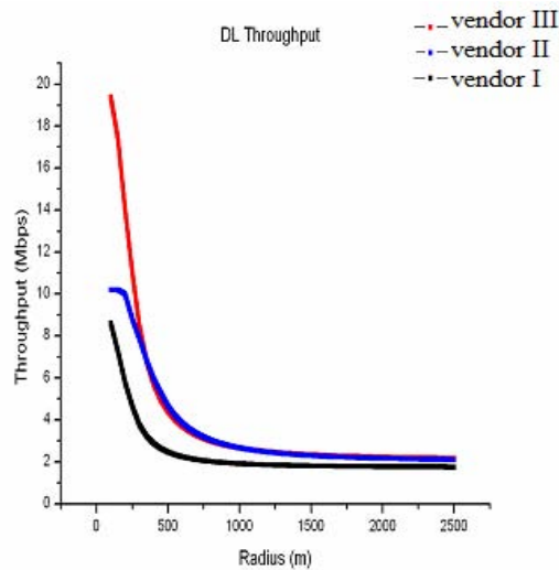
Figure 10.3 Throughput per sector versus radius of cell for DL direction
