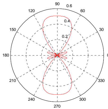
Figure 5.13 Beamforming of AP 2 and 4 scenario B
