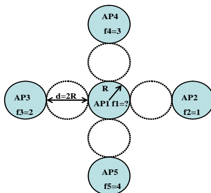
Figure 6.1 Deployment of a configuration
