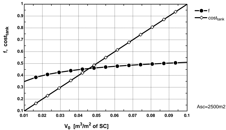
Figure 23: Variation of load cover fraction f & unit cost of the storage tank per its volume (for the case of A_{SC} = 2500m^2 )
