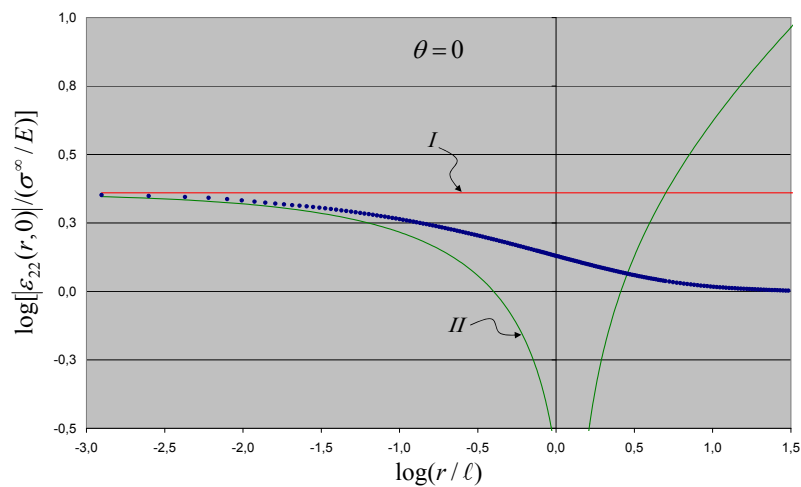
Figure 4.11: Variation of \log \frac{|\varepsilon_{22}|}{\sigma_{\infty}/E} ahead of the crack ( \theta = 0 ). Curve I represents the leading term in the asymptotic expansion of the solution, curve II is the sum of the first two terms in the expansion, and the dots are the results of the finite element solution.
