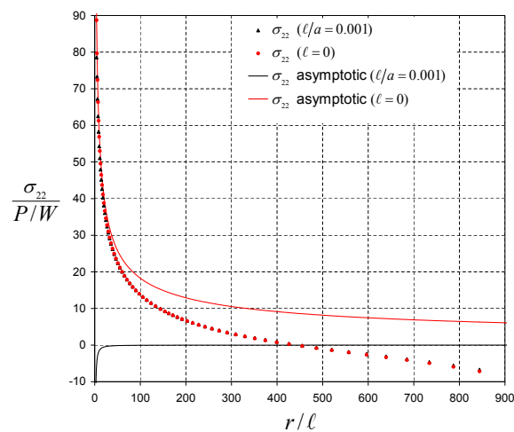
Figure 5.16: Variation of the normalized true stress \sigma_{22}/(P/W) as a function of the normalized radial distance r/l along the radial line \theta = \frac{\pi}{40} for both the gradient and classical elasticity solutions.
