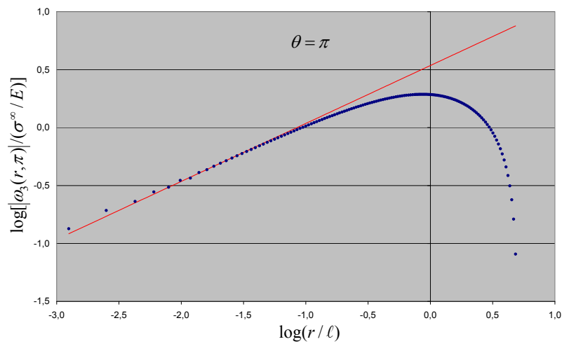
Figure 4.8: Variation of \log \frac{|\omega_3(r, \pi)|}{\sigma^\infty / E} with \log \frac{r}{\ell} along the crack face ( \theta = \pi ). The solid line represents the asymptotic crack-tip solution, and the dots the results of the finite element solution.
