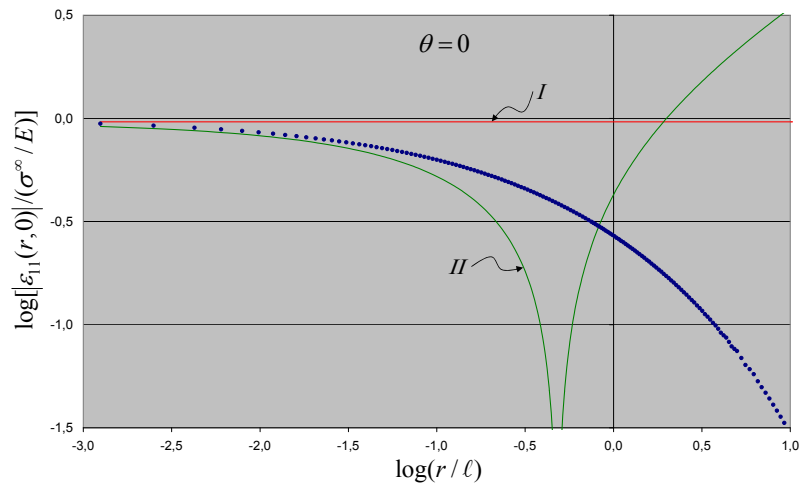
Figure 4.10: Variation of \log \frac{|\varepsilon_{11}|}{\sigma_{\infty}/E} ahead of the crack ( \theta = 0 ). Curve I represents the leading term in the asymptotic expansion of the solution, curve II is the sum of the first two terms in the expansion, and the dots are the results of the finite element solution.
