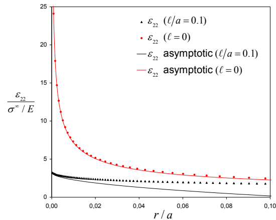
Figure 4.23: Variation of the normalized normal strain \epsilon_{22}/(\sigma^\infty/E) as a function of the normalized radial distance r/a along the radial line \theta = 0 for both the gradient and classical elasticity solutions.
