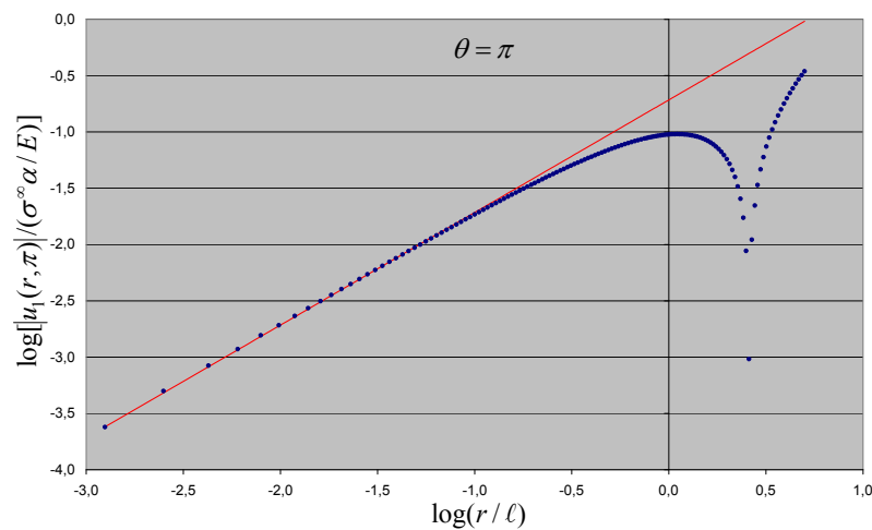
Figure 4.6: Variation of \log \frac{u_1}{\sigma_\infty a / E} with \log \frac{r}{\ell} along the crack face ( \theta = \pi ). The solid line represents the asymptotic crack-tip solution, and the dots the results of the finite element solution.
