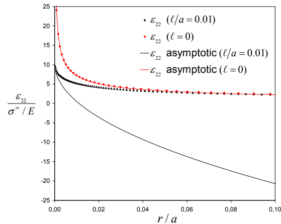
Figure 4.24: Variation of the normalized normal strain \epsilon_{22}/(\sigma^\infty/E) as a function of the normalized radial distance r/a along the radial line \theta = 0 for both the gradient and classical elasticity solutions.
