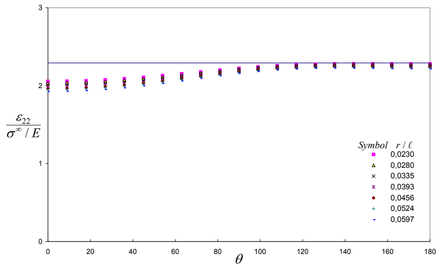
Figure 4.15: Angular variation of \frac{\varepsilon_{22}}{\sigma^\infty/E} at various radial distances. The solid line represents the asymptotic crack-tip solution.
