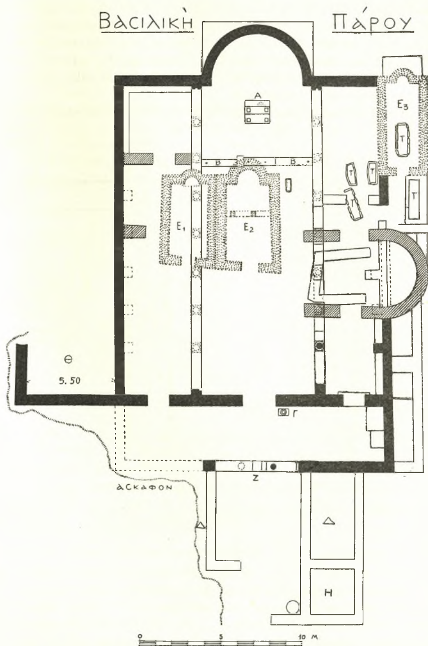
Εἰκ. 1. Κάτοπις τῆς βασιλικῆς τῶν Τριῶν Ἐκκλησιῶν τῆς Πάρου
