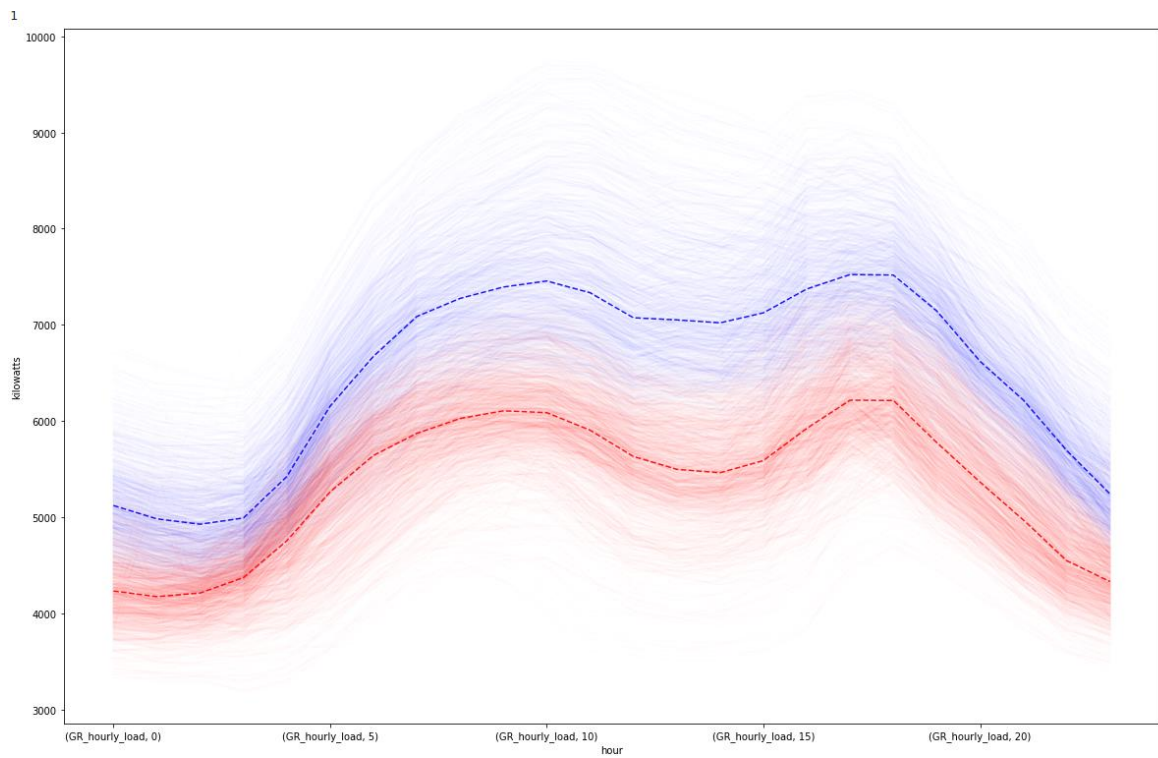
Figure 5.13: Selected clusters
