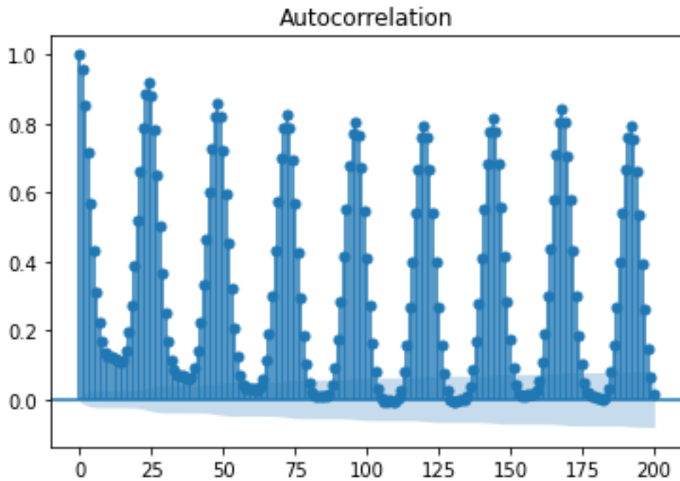
5.4: Autocorrelation graph
