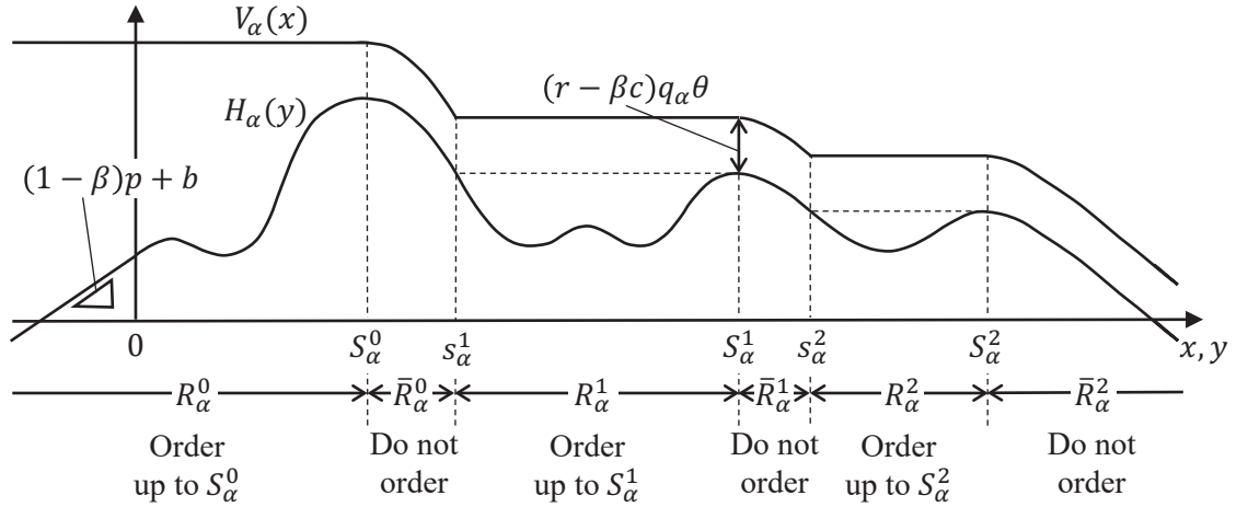
Figure 2.1: Optimal inventory control policy.
