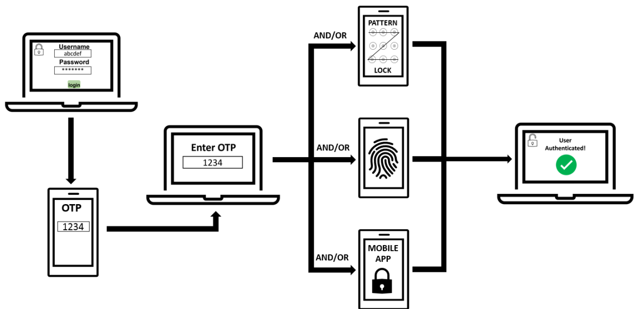
Figure 3: Multifactor authentication.
