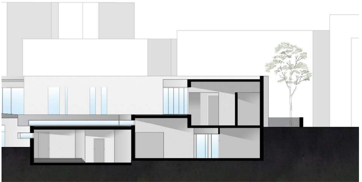
ΤΟΜΗ Α'' Α''
