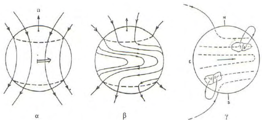
Fig.11. Dynamic lines of the solar magnetic field.
