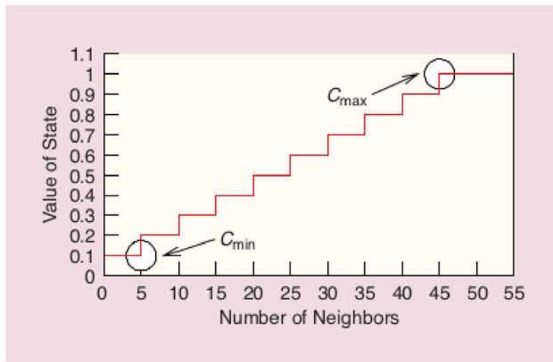
Figure 4.4: State mapping according to the number of neighboring vehicles
