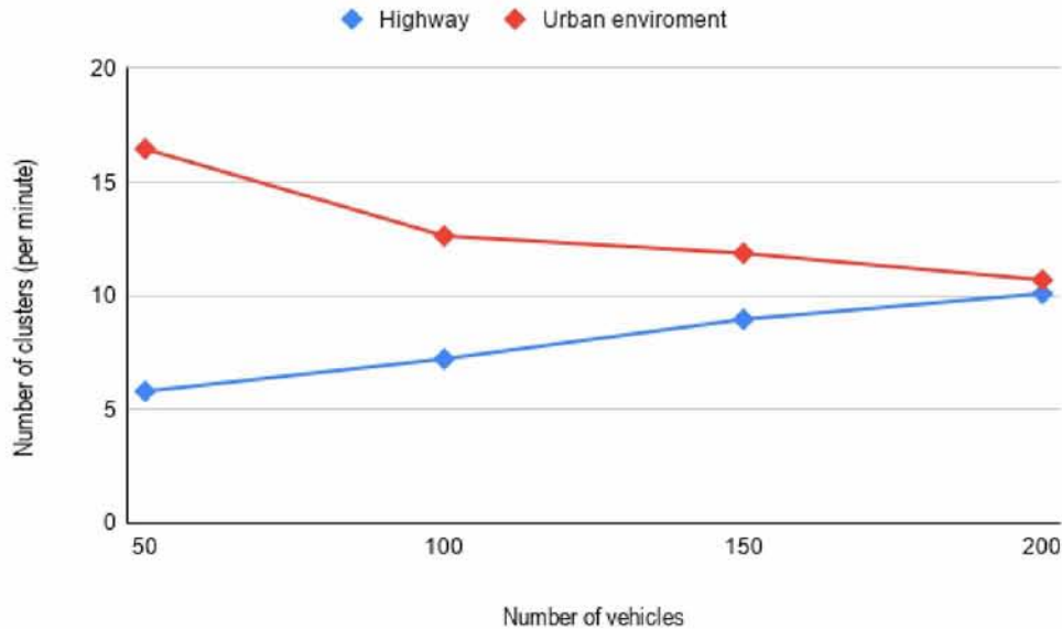
Figure 5.4: Number of clusters (per minute) for various number of vehicles. Blue line: Highway model and red line: Urban environment, respectively
