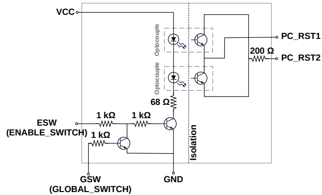
Figure 6.2: Complementary circuit for resetting the target platform.
