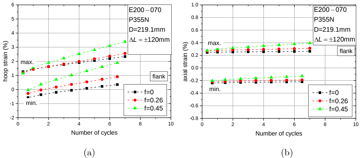
Figure 35. Evolution of maximum and minimum strain at the elbow flank [SCH 40]; (a) hoop strain, (b) axial strain.
