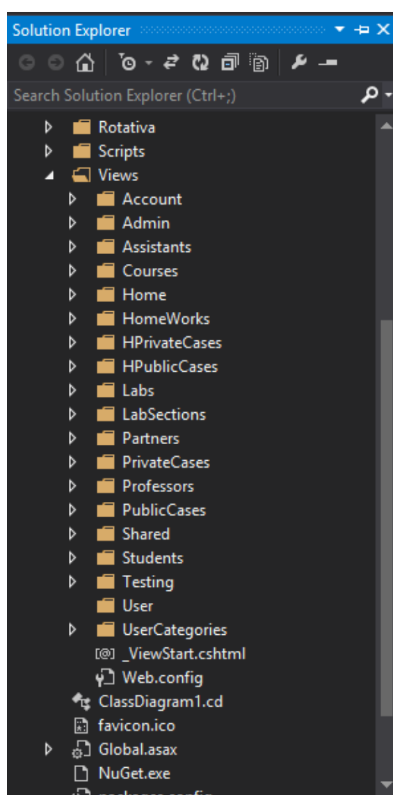
Figure 14. Application Views
