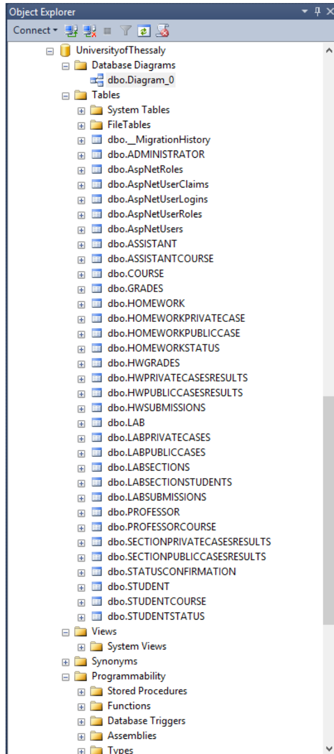
Figure 9. Database Tables
