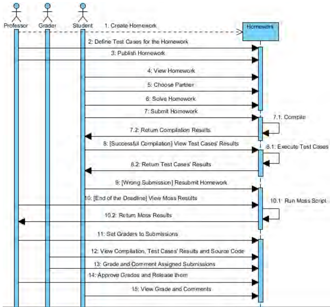
Figure 4. The Life of a Homework - UML Sequence Diagram
