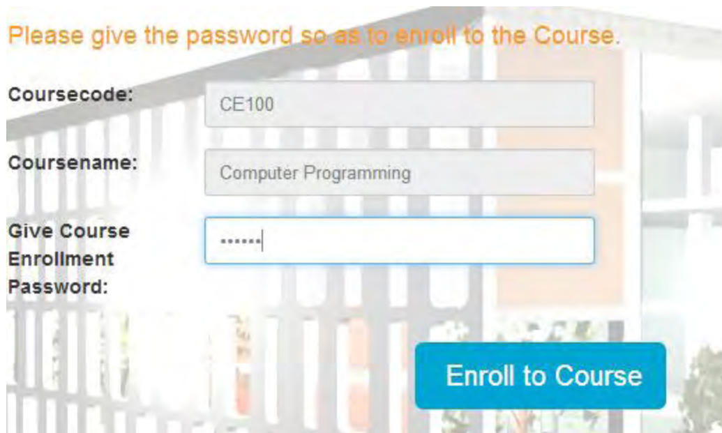
Figure 47. Course Enrollment
