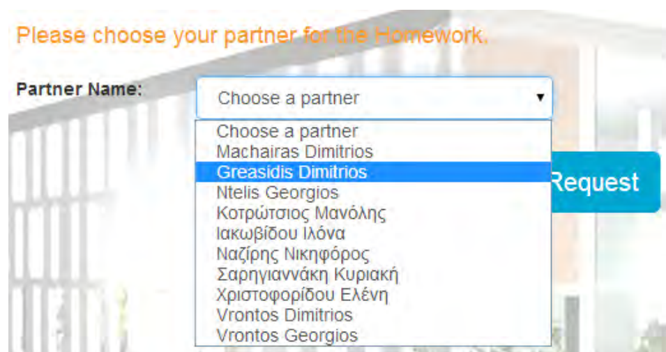
Figure 51. Partner's Choice
