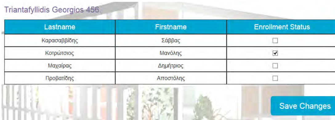
Figure 37. Grader Choice
