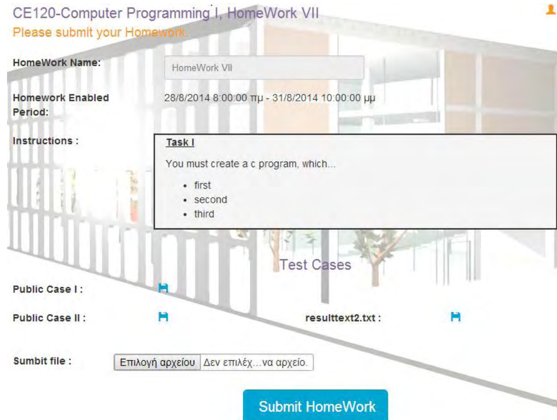
Figure 50. Homework Task
