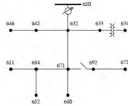
FIGURE 5.2: The IEEE-13 test feeder.
