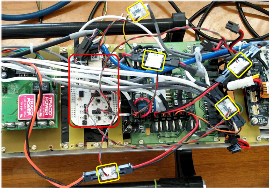
FIGURE 5.2: LAUV vehicle installation
