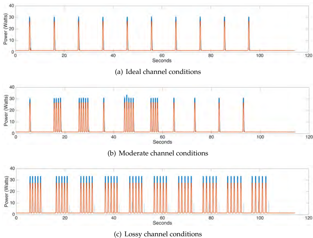
FIGURE 6.2: Power consumption of Evologics S2CR18/34 modem under various channel conditions
