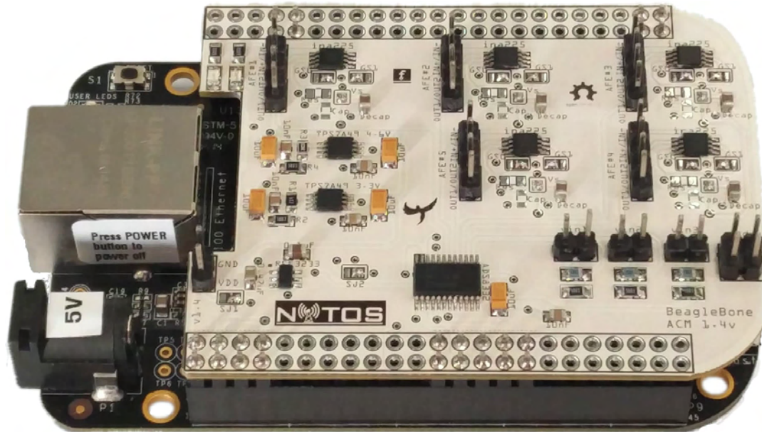
FIGURE 5.3: Developed power monitoring device
