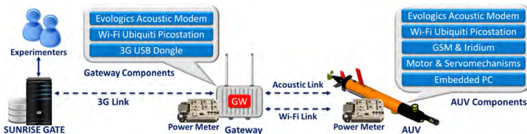
FIGURE 5.1: The power consumption monitoring framework, integrated with the SUNRISE testbed
