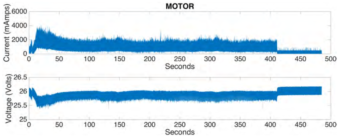
FIGURE 6.4: LAUV motor power consumption
