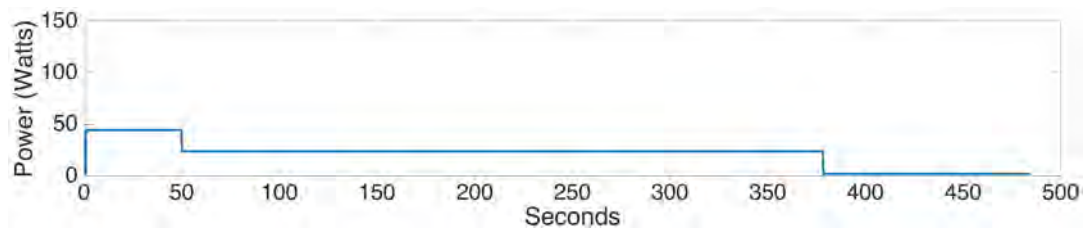
FIGURE 6.5: Simulated LAUV motor power consumption
