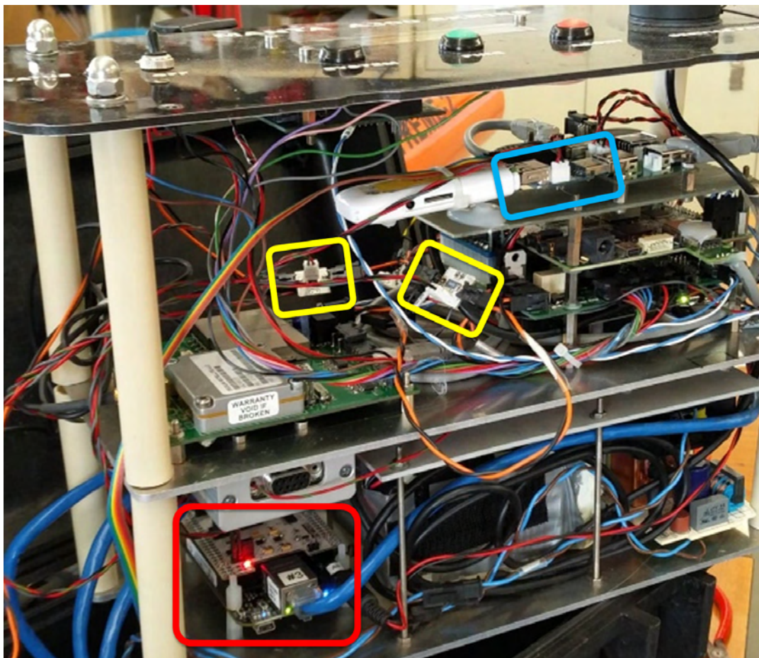
FIGURE 5.4: Manta gateway installation
