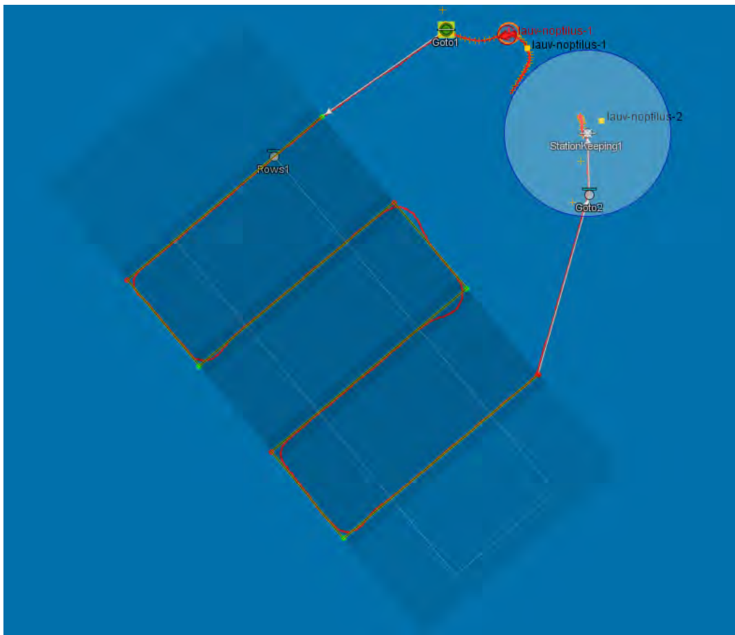
FIGURE 6.3: LAUV route
