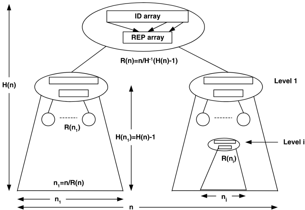
Σχήμα 4.1: Static Interpolation Search Tree - SIST, [6]
