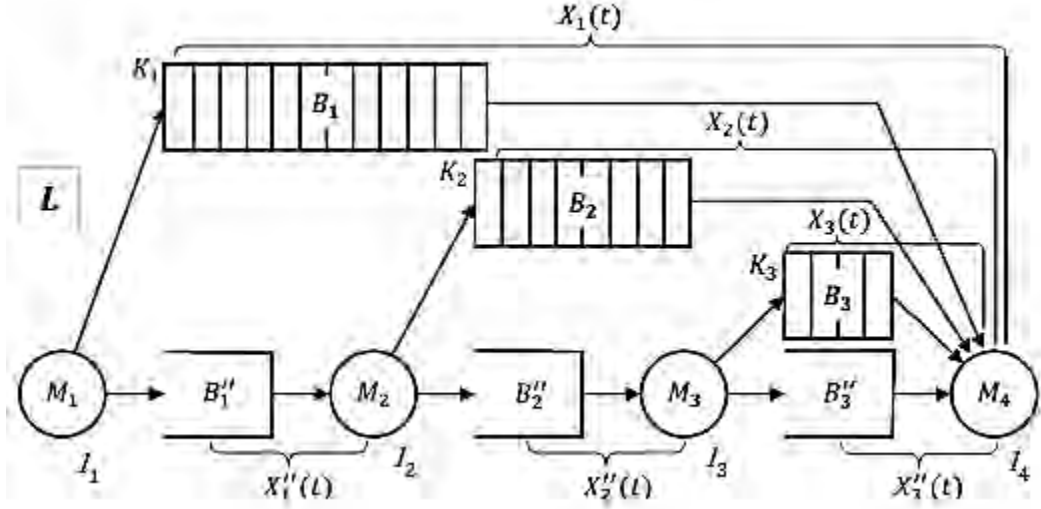
Figure 4. Queueing network model of a serial production line operated under an EB policy.
