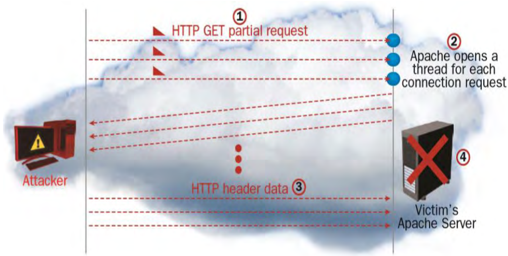
figure19, Slow HTTP GET Request
