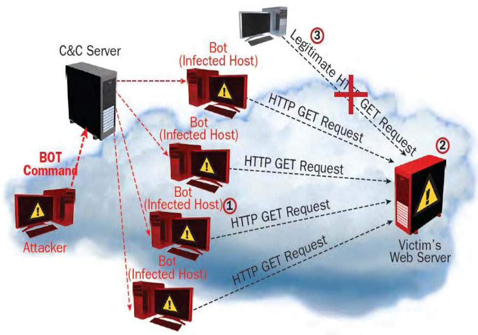
Figure18, HTTP Flood
