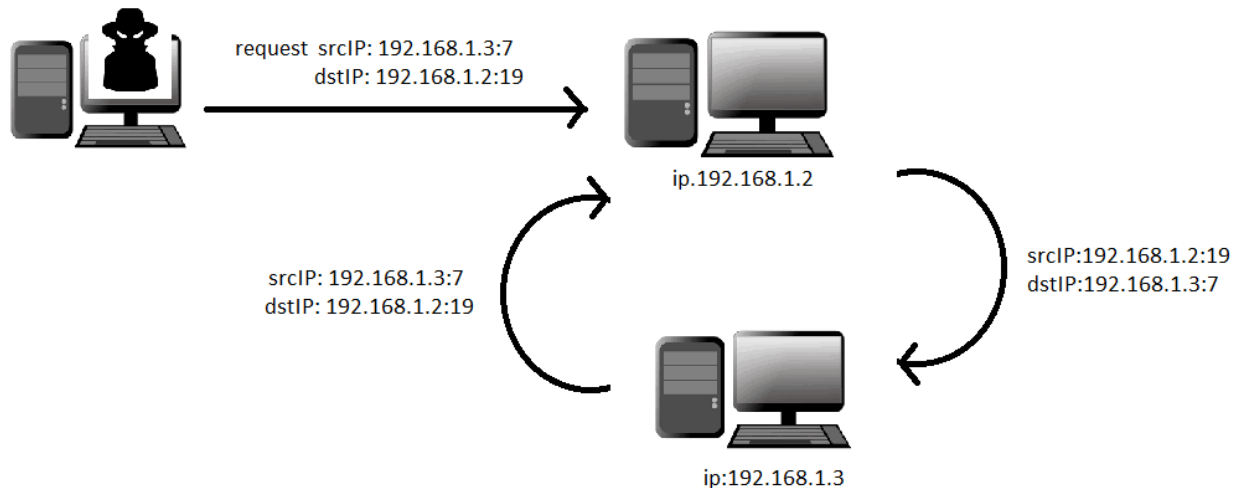
figure12, fraggle attack
