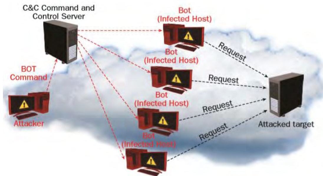
figure.1, Botnet Infrastructure
