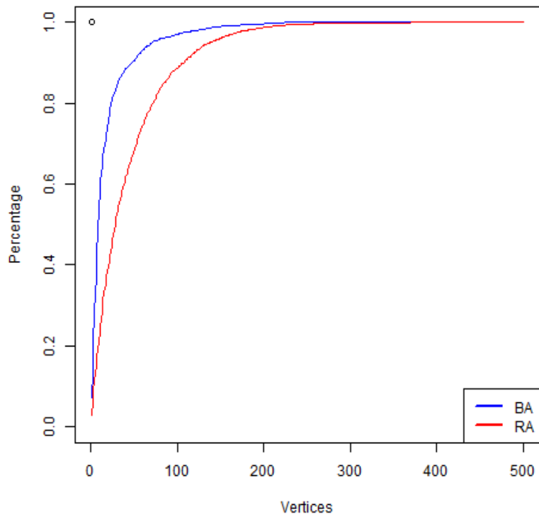
Cover rate function for HDF
