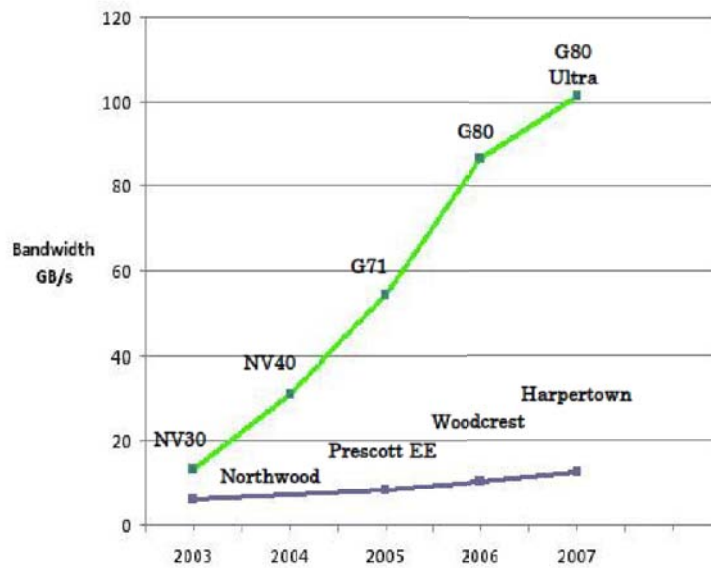
FIGURE 3.1: Floating point operations per second and memory bandwidth for the CPU and GPU.
