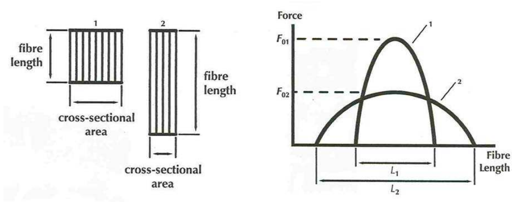
Figure 2.17: Force-length relationship of two muscles with different cross-sectional areas and fiber length, but equal volume. (From Nigg and Herzog, 1999)
