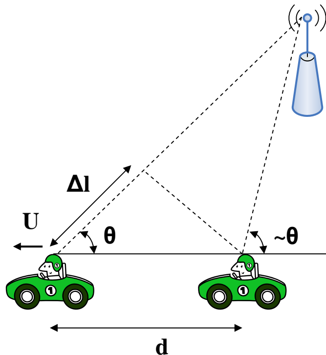
Figure 3.1 Doppler effect
