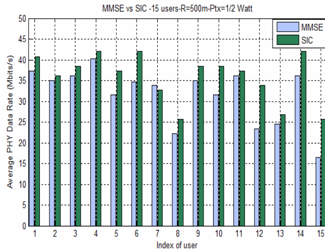
Figure 9.15 MMSE versus SIC
