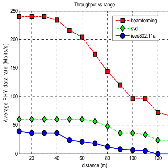
Figure 5.10 Throughput versus range for LOS/NLOS channel
