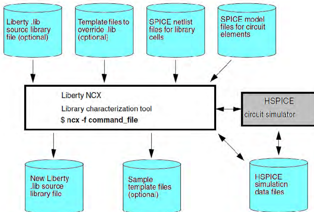
Figure 9 : Liberty NCX Characterization Data
