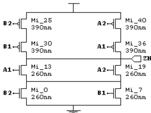
Figure 11: Schematic of cell OAI22_X2
