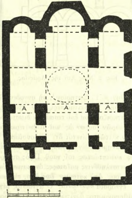
Εἰκ. 1. Ἡ κάτοπις τοῦ ναοῦ Ἁγ. Θεοδώρου τῶν Κυθήρων.
