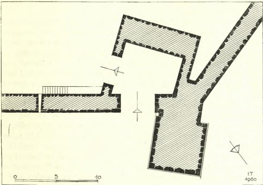
Εἰκ. 1. Κάτοψις τῶν Ἀστυδε Πυλῶν.
