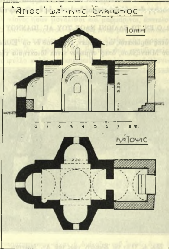
Εἰκ. 5. Κάτοψις καὶ τομή τοῦ ἐν τῷ Ἐλαιῶνι ναοῦ.
