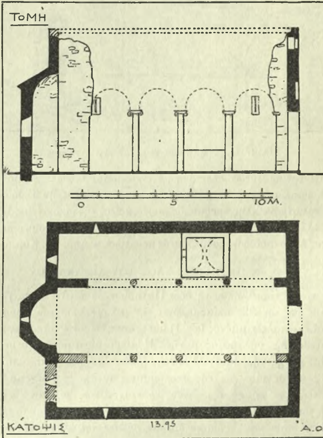
Εἰκ. 2. Κάτοψις καὶ τομὴ τοῦ ἐν Πατησίοις ναοῦ τοῦ Ἁγ. Ἀνδρέου.
