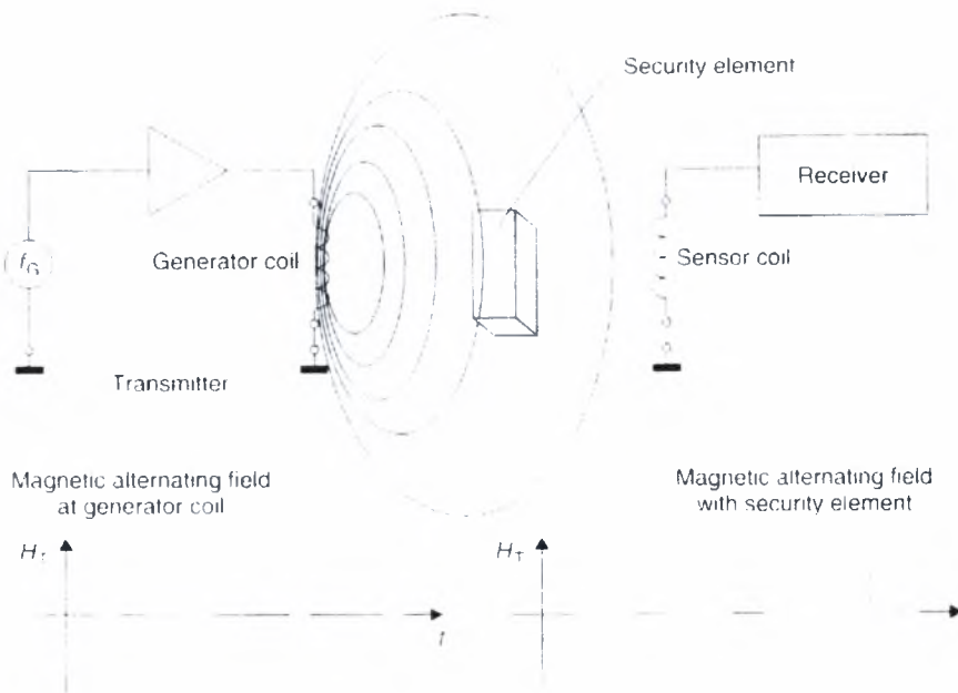
Figure 2.5: Acoustomagnetic system comprising transmitter and detection device (receiver). If a security element is within the field of the generator coil, this oscillates like a tuning fork in time with the pulses of the generator coil. The transient characteristics can be detected by an analyzing unit.
