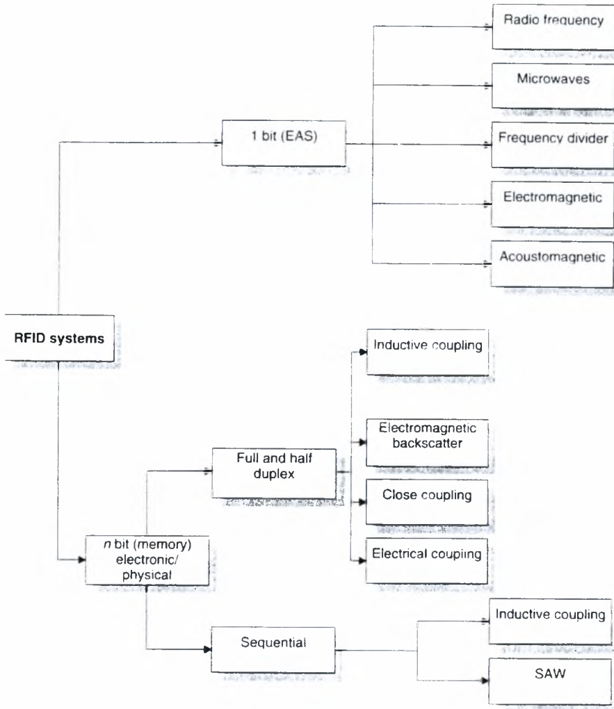
Figure 2.1: The different operating principles of RFID systems.
