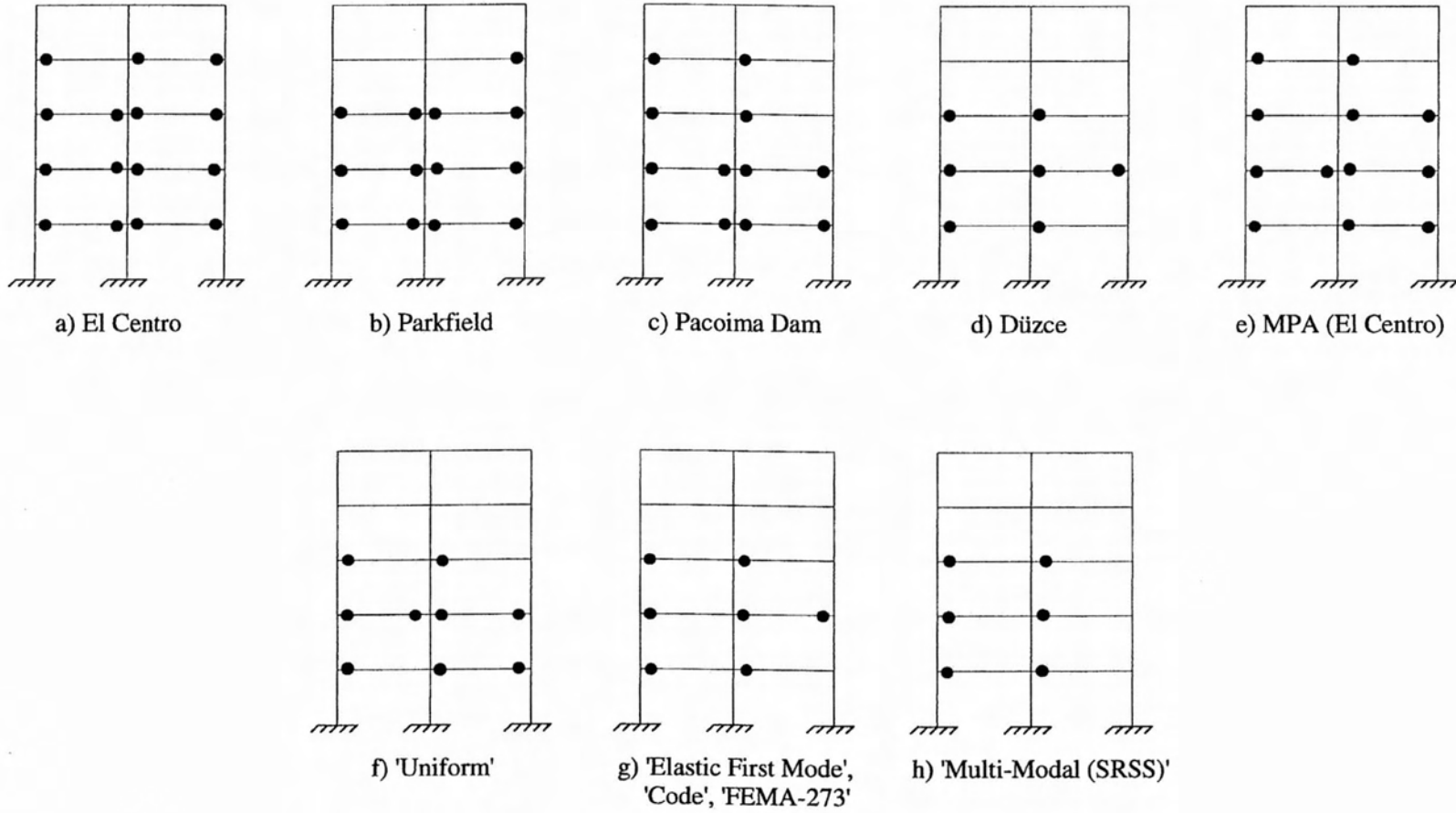
Figure A.15 : Plastic Hinges for 5-Story R/C Frame (Deformation Level II)
