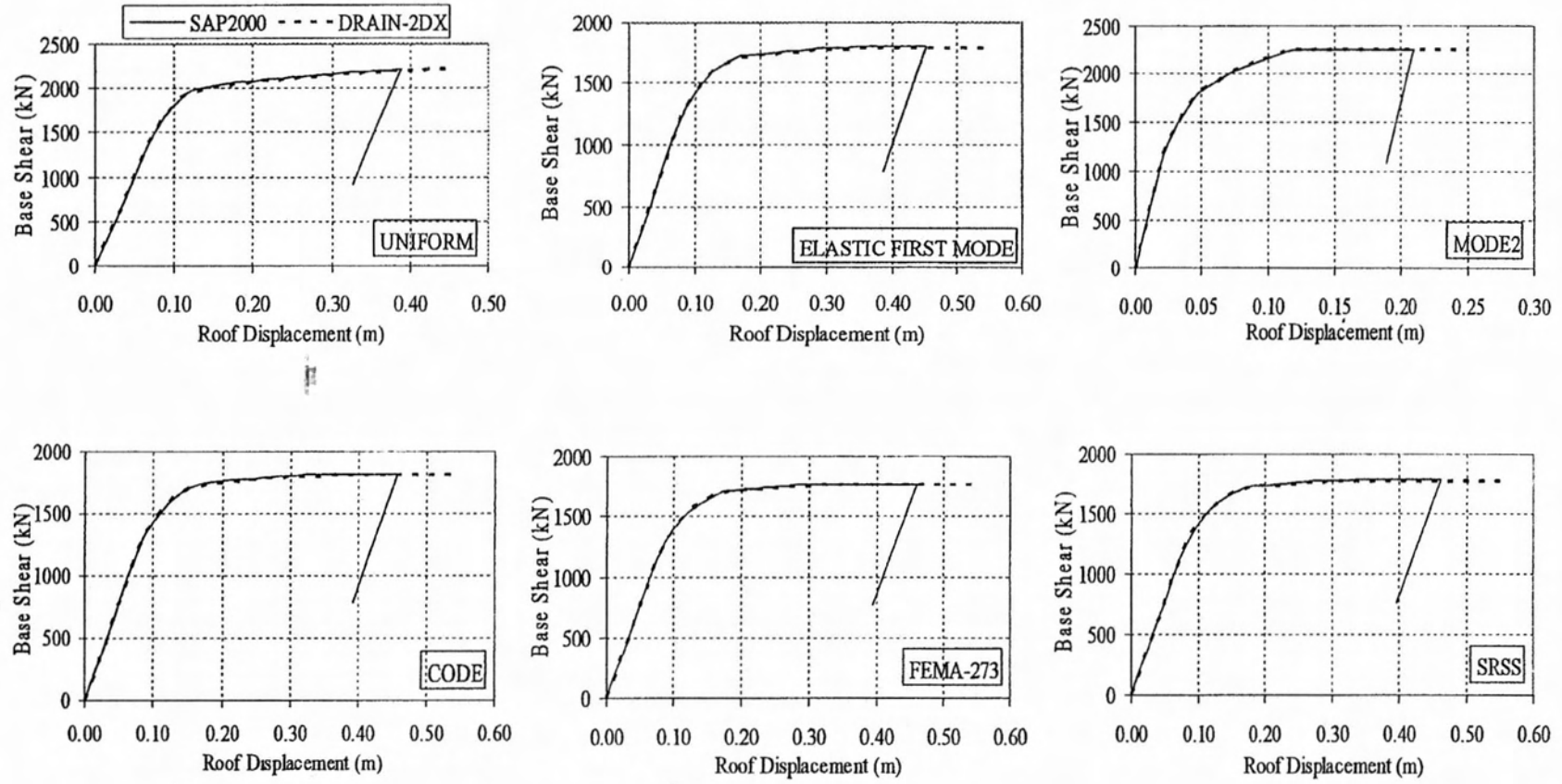
Figure 3.17 : Pushover (Capacity) Curves for 5-Story R/C Frame
