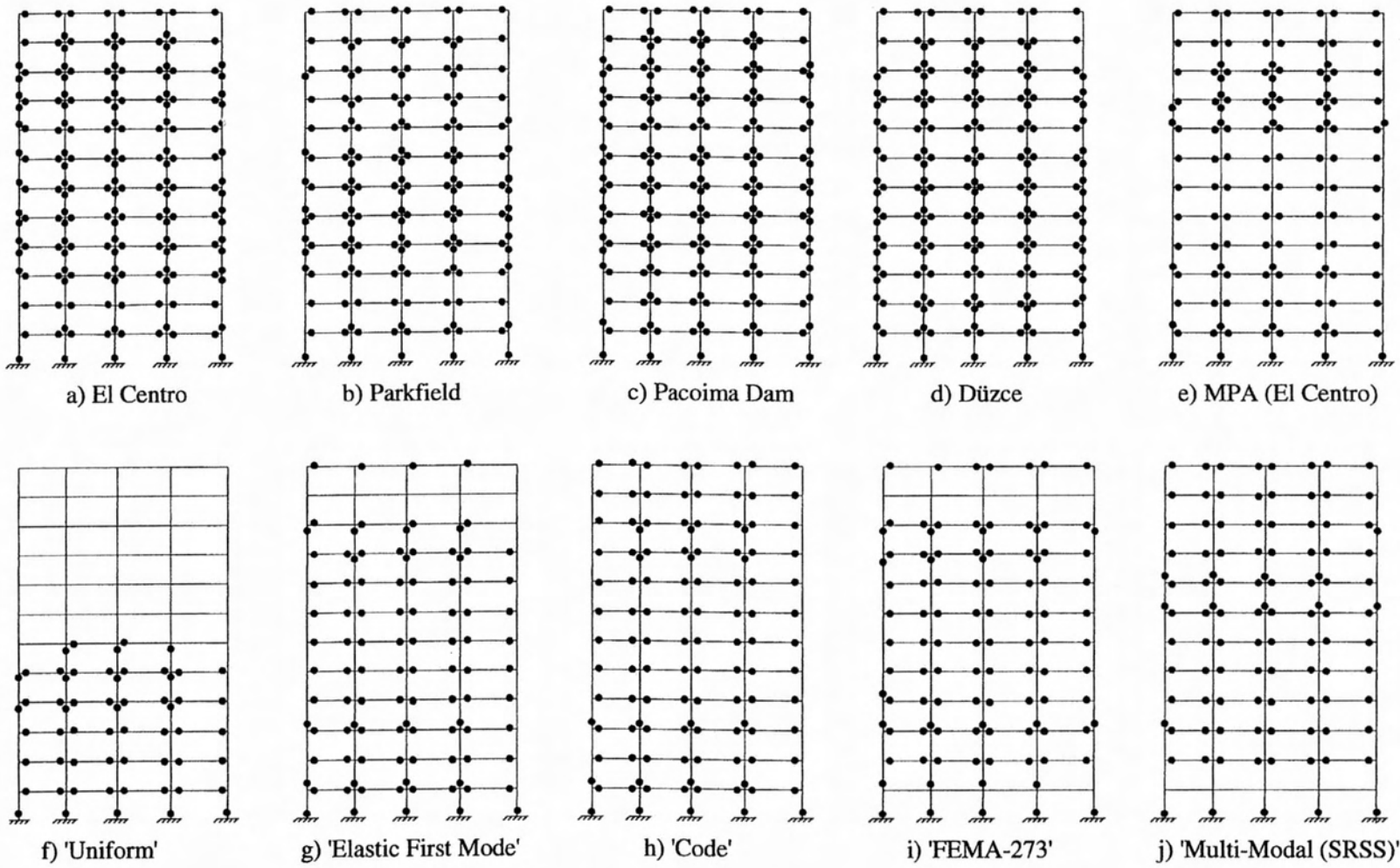
Figure A.20 : Plastic Hinges for 12-Story R/C Frame (Deformation Level VI)
