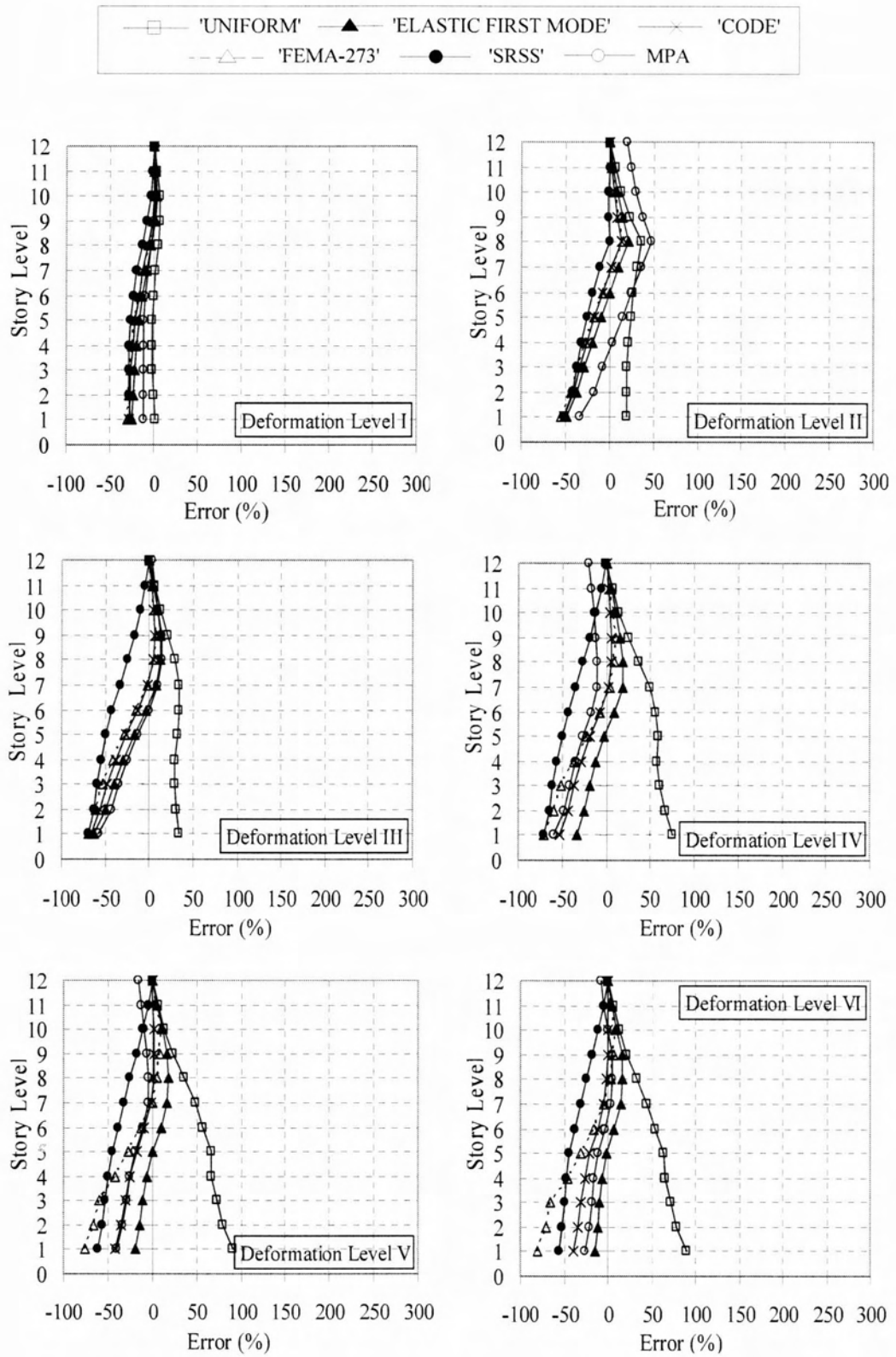
Figure 4.16 : Story Displacement Error Profile for 12-Story R/C Frame (Parkfield)
