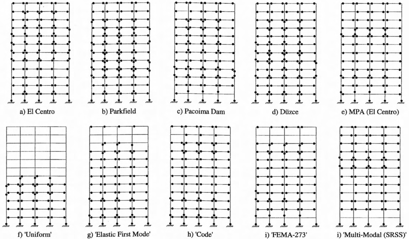
Figure A.19 : Plastic Hinges for 12-Story R/C Frame (Deformation Level III)
