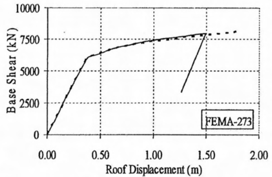
Figure 3.15 : Pushover (Capacity) Curves for 13-Story Steel Frame
