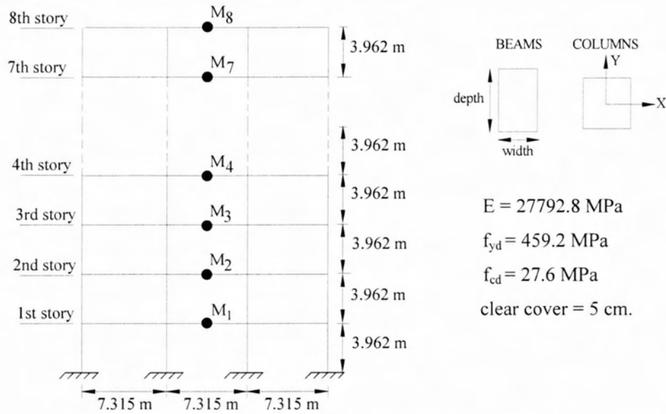
Figure A.3 : The Configuration of 8-Story Reinforced Concrete Frame
