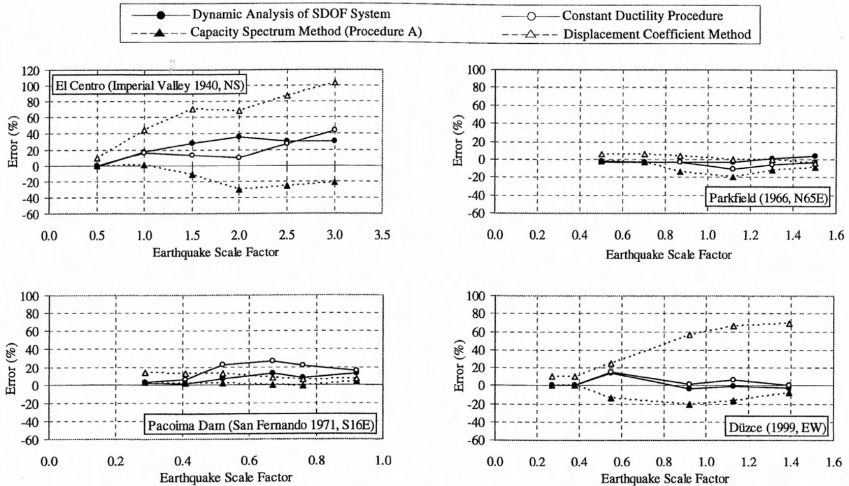
Figure 5.10 : Error in Target Displacement Estimation for 5-Story R/C Frame
