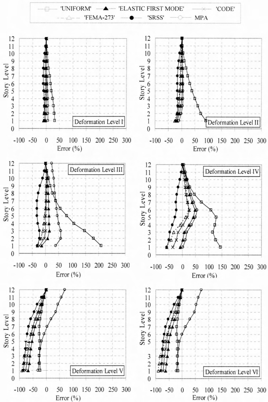
Figure 4.18 : Story Displacement Error Profile for 12-Story R/C Frame (Düzce)
