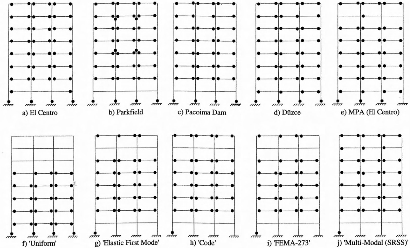
Figure 4.33 : Plastic Hinges for 8-Story R/C Frame (Deformation Level III)
