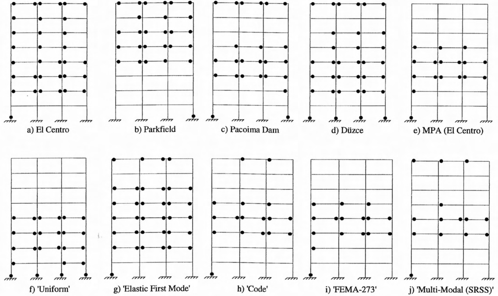
Figure 4.32 : Plastic Hinges for 8-Story R/C Frame (Deformation Level II)
