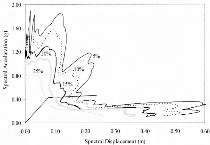
Figure 5.8 : Capacity Spectrum Method (ATC-40 Procedure A)
