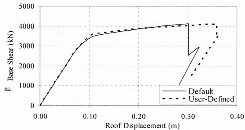
Figure 3.10 : Pushover Curves Obtained Using Default and User-Defined Hinge Properties for 5-Story R/C Frame Under 'Uniform' Lateral Load Pattern
