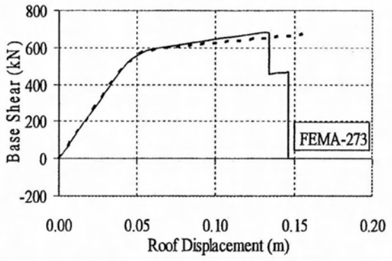
Figure 3.13 : Pushover (Capacity) Curves for 2-Story Steel Frame
