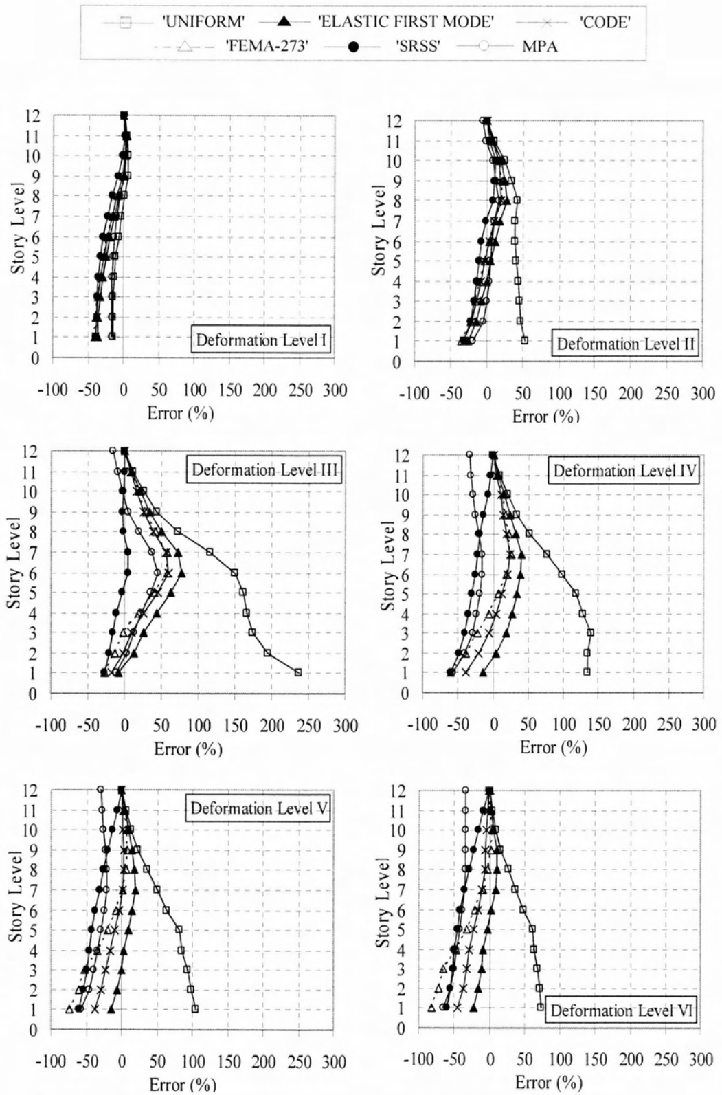
Figure 4.15 : Story Displacement Error Profile for 12-Story R/C Frame (El Centro)
