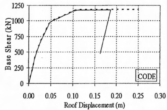
Figure 3.16 : Pushover (Capacity) Curves for 2-Story R/C Frame
