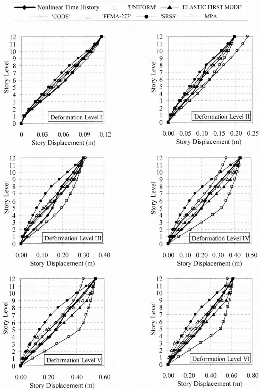
Figure 4.12 : Story Displacement Profile for 12-Story R/C Frame (Parkfield)
