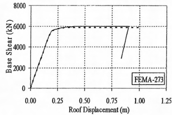
Figure 3.19 : Pushover (Capacity) Curves for 12-Story R/C Frame
