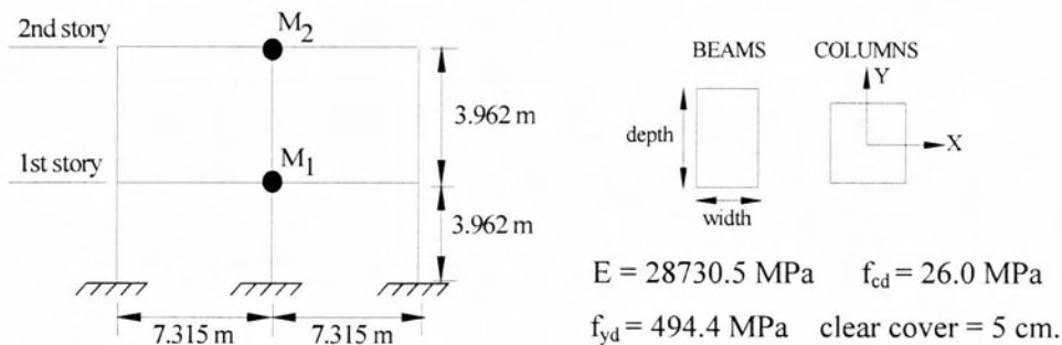
Figure A.1 : The Configuration of 2-Story Reinforced Concrete Frame
