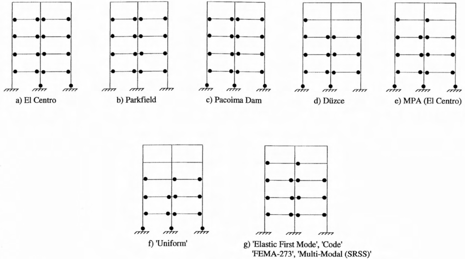
Figure A.16 : Plastic Hinges for 5-Story R/C Frame (Deformation Level III)
