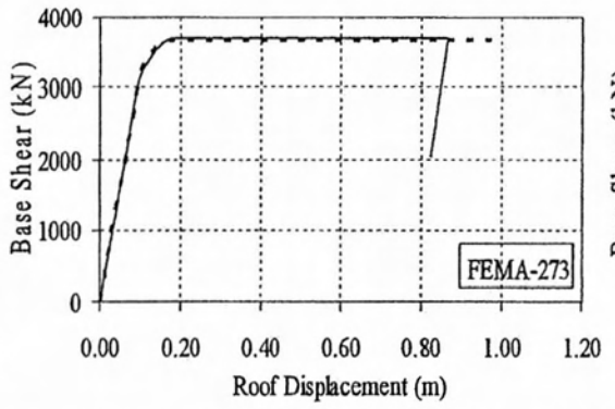
Figure 3.18 : Pushover (Capacity) Curves for 8-Story R/C Frame
