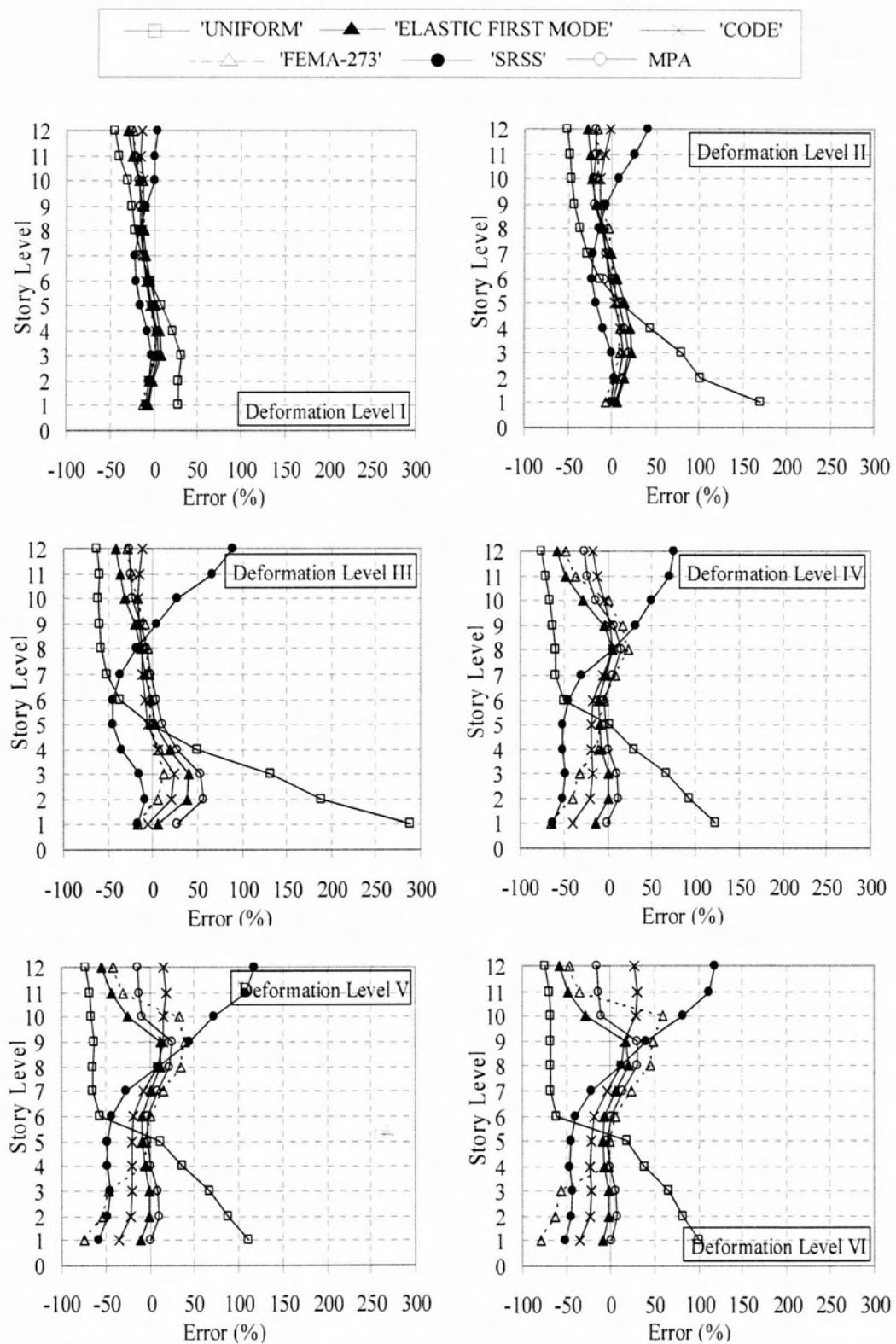
Figure 4.25 : Inter-Story Drift Ratio Error Profile for 12-Story R/C Frame (Pacoima Dam)
