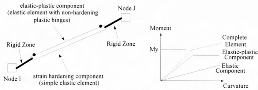
Figure 3.2 : Geometry and Moment-Curvature Relationship of "Type 02" Element
