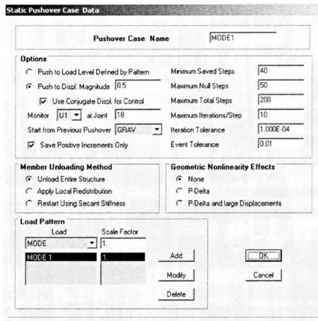
Figure 3.4 : Static Pushover Case Data Dialog Box (SAP2000)
