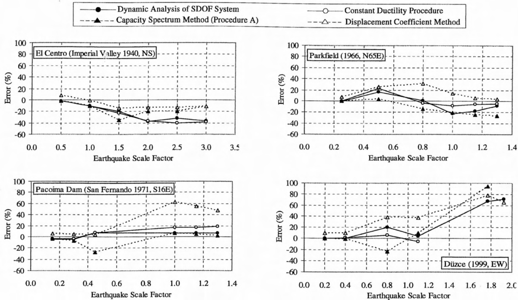
Figure 5.12 : Error in Target Displacement Estimation for 12-Story R/C Frame
