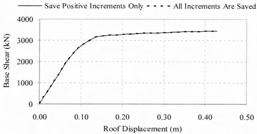
Figure 3.7 : Member Unloading Method-"Apply Local Redistribution"
