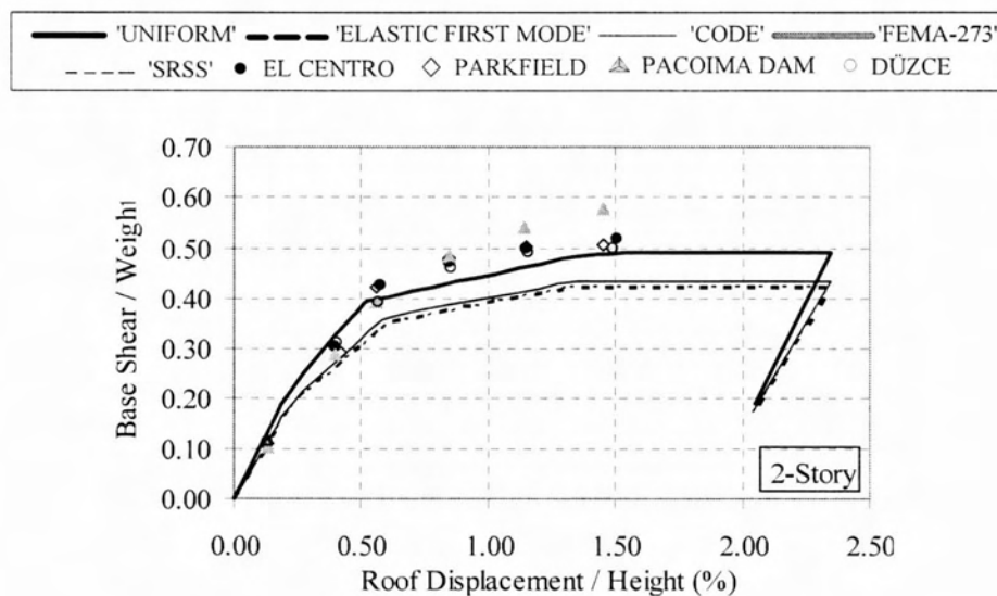
Figure 4.8 : Capacity (Pushover) Curves (2-Story R/C Frame)
