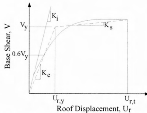
Figure 5.2 : Bilinear Representation of Capacity (Pushover) Curve
