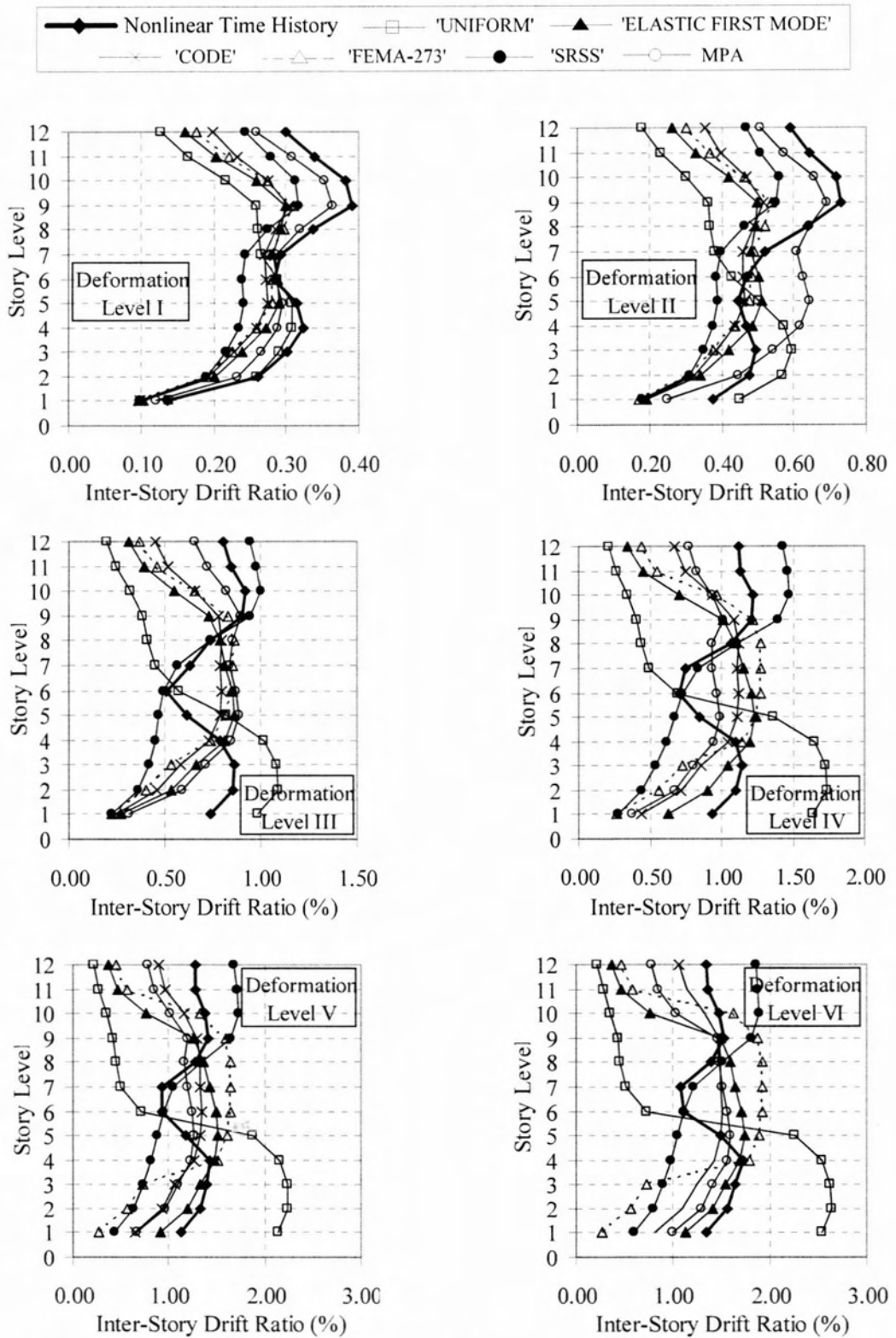
Figure 4.20 : Inter-Story Drift Ratio Profile for 12-Story R/C Frame (Parkfield)
