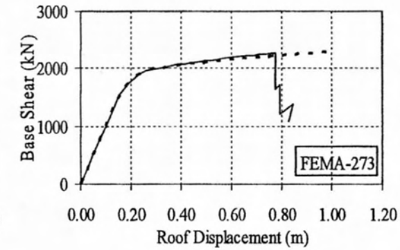
Figure 3.14 : Pushover (Capacity) Curves for 5-Story Steel Frame
