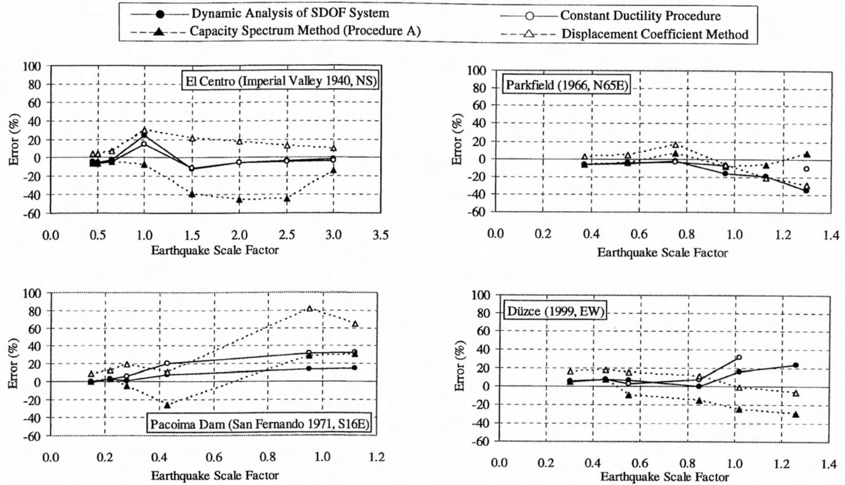
Figure 5.11 : Error in Target Displacement Estimation for 8-Story R/C Frame
