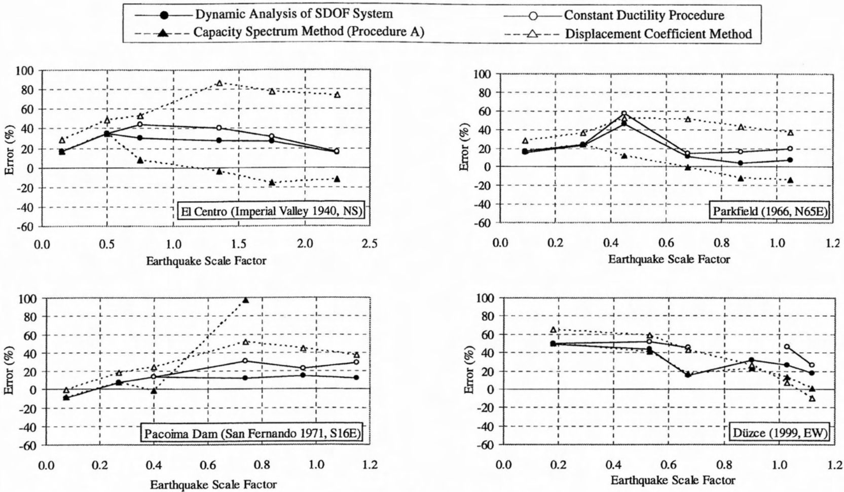
Figure 5.9 : Error in Target Displacement Estimation for 2-Story R/C Frame
