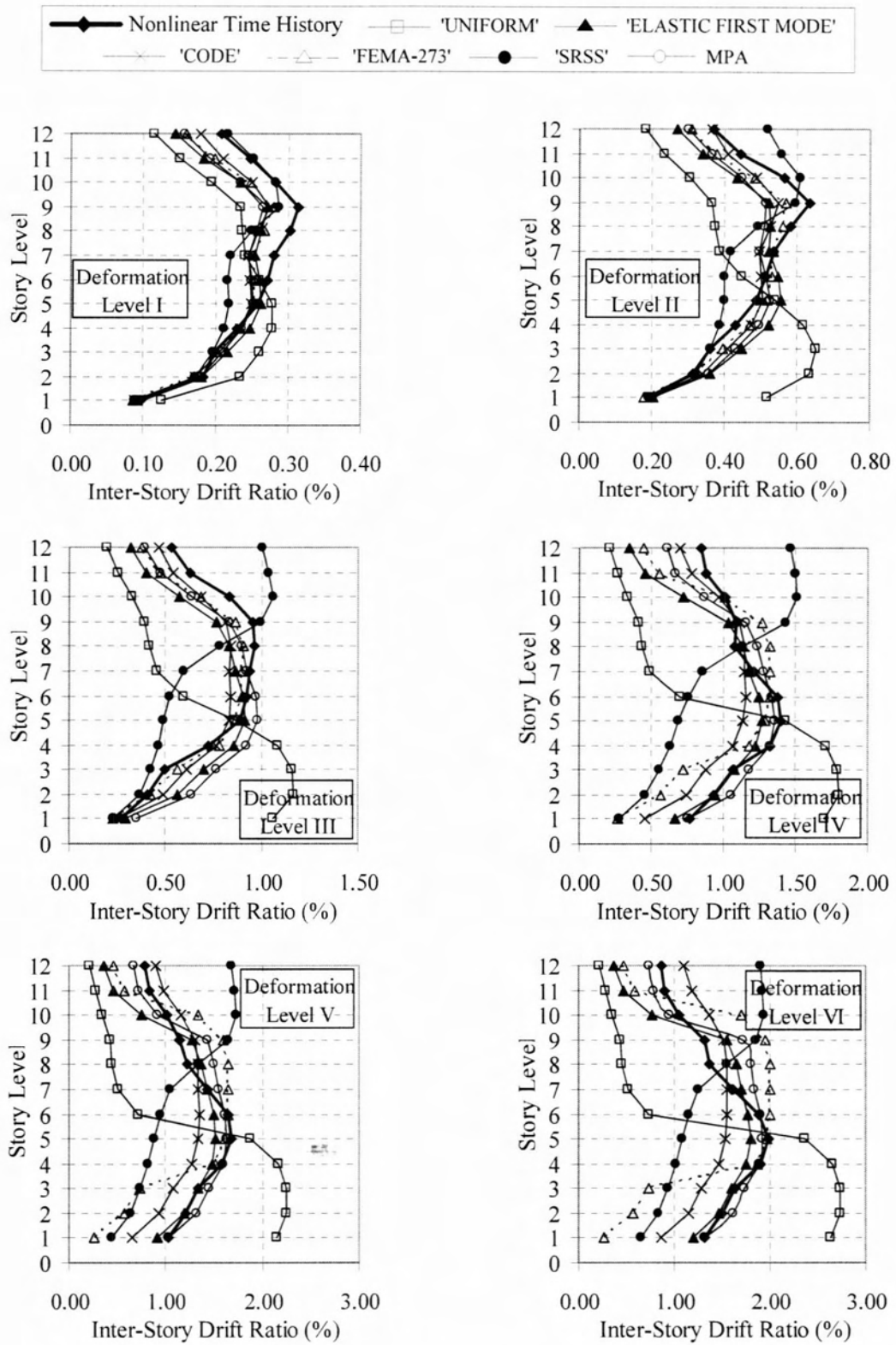
Figure 4.21 : Inter-Story Drift Ratio Profile for 12-Story R/C Frame (Pacoima Dam)
