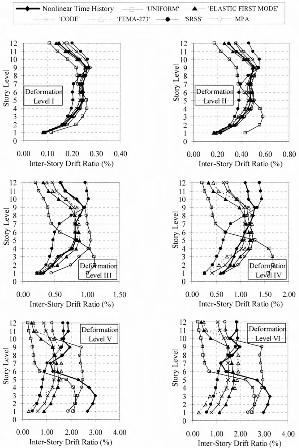
Figure 4.22 : Inter-Story Drift Ratio Profile for 12-Story R/C Frame (Düzce)
