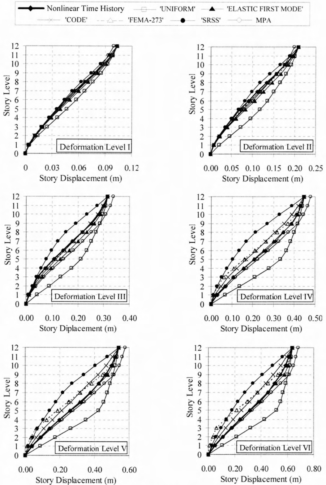
Figure 4.13 : Story Displacement Profile for 12-Story R/C Frame (Pacoima Dam)
