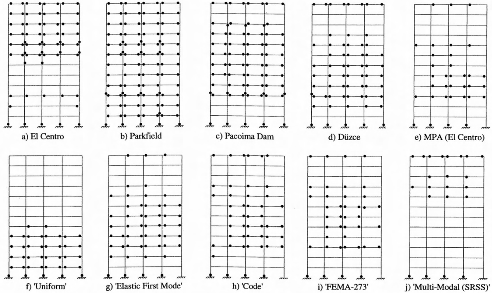
Figure A.18 : Plastic Hinges for 12-Story R/C Frame (Deformation Level II)
