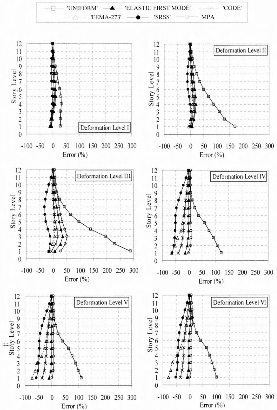
Figure 4.17 : Story Displacement Error Profile for 12-Story R/C Frame (Pacoima Dam)
