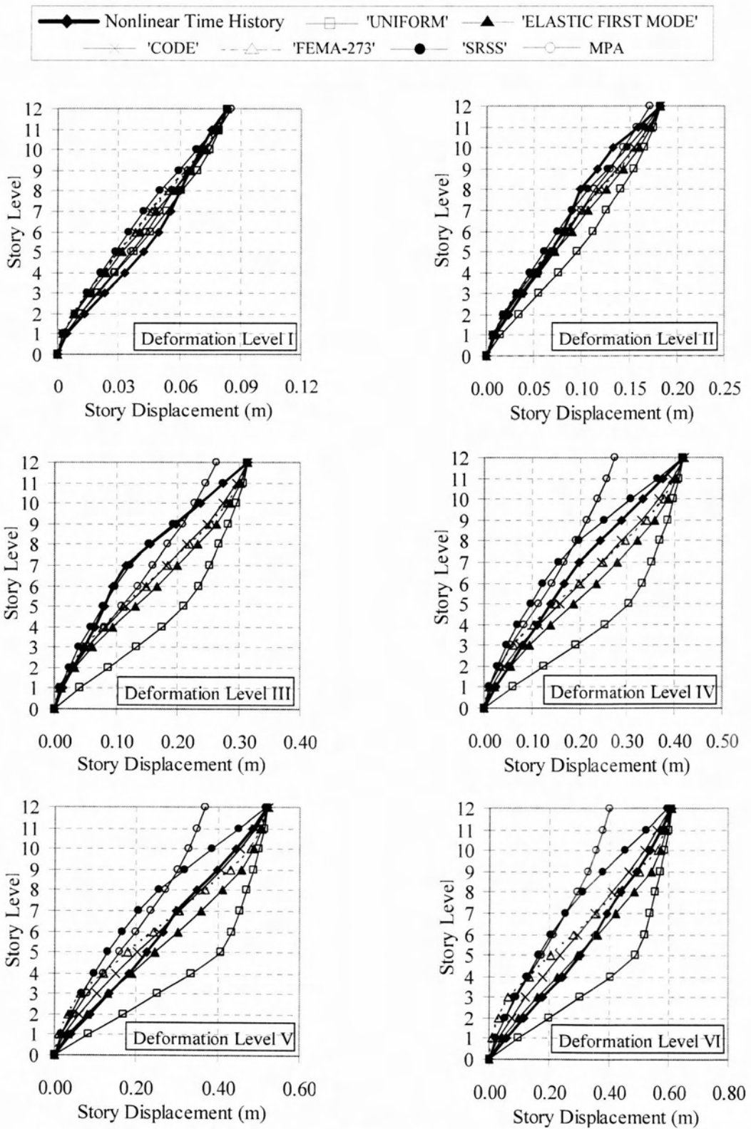
Figure 4.11 : Story Displacement Profile for 12-Story R/C Frame (El Centro)
