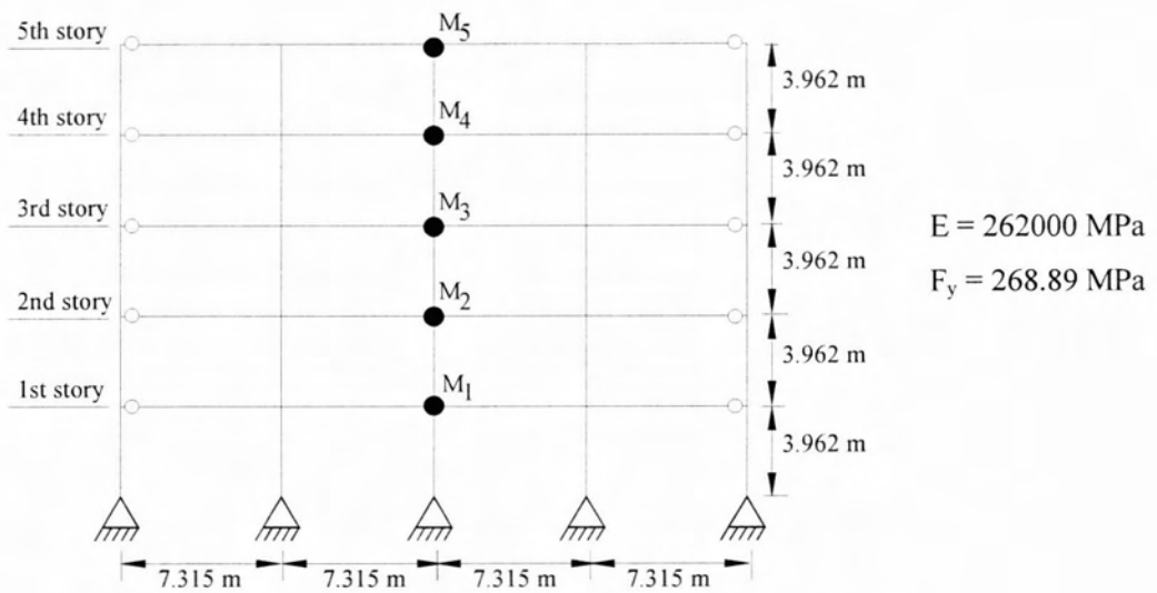
Figure A.6 : The Configuration of 5-Story Steel Frame
