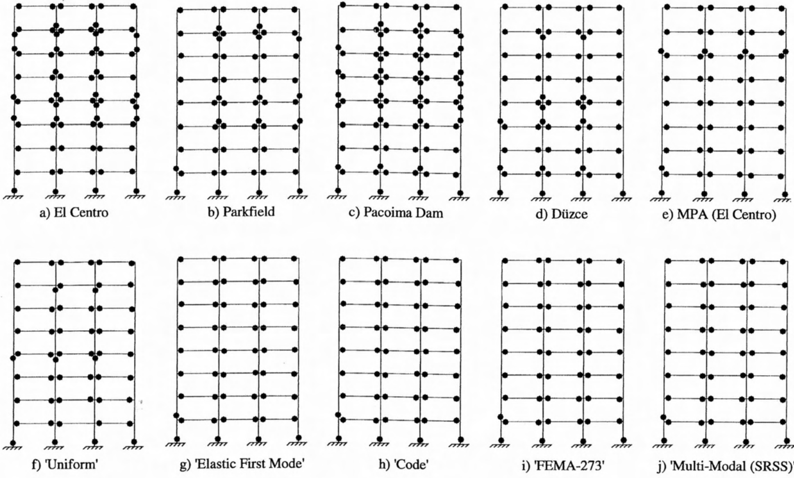
Figure 4.34 : Plastic Hinges for 8-Story R/C Frame (Deformation Level VI)
