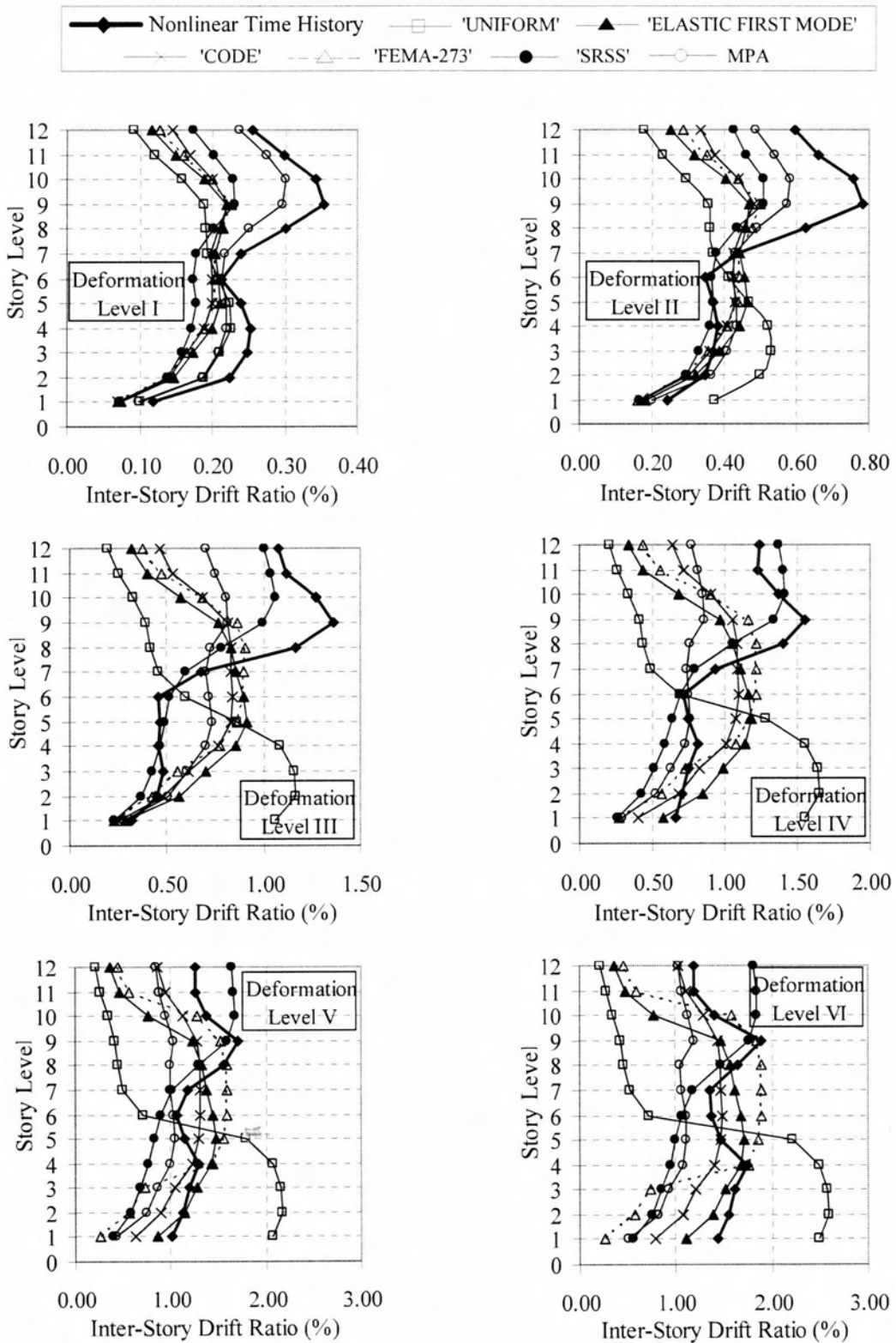
Figure 4.19 : Inter-Story Drift Ratio Profile for 12-Story R/C Frame (El Centro)
