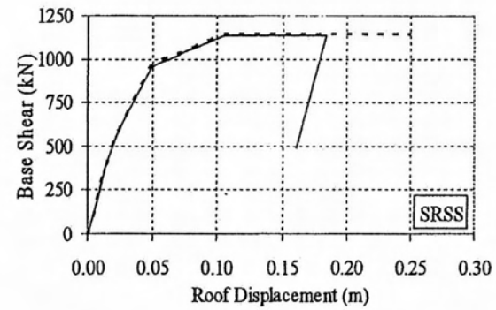
Figure 3.16 : Pushover (Capacity) Curves for 2-Story R/C Frame
