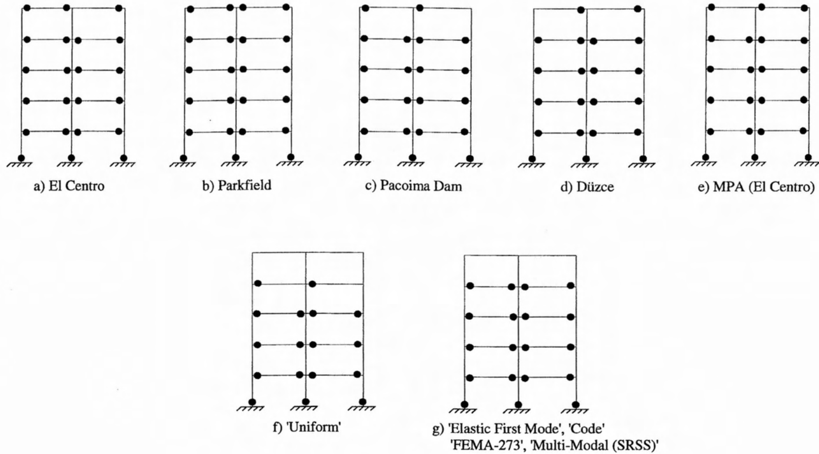
Figure A.17 : Plastic Hinges for 5-Story R/C Frame (Deformation Level VI)
