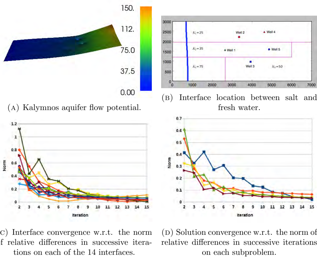
FIGURE 8.2: Results and convergence for 15 iterations of the Schwarz method.
