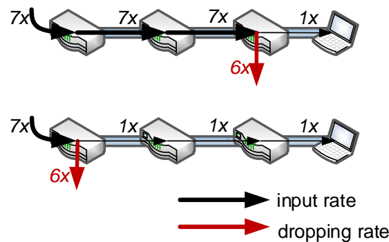
Figure 4.1: An example of an overloaded network where distributed load shedding (top) may consume more energy than source-based congestion control (bottom). We propose a novel load shedding mechanism which minimizes energy usage by adjusting real-time dropping decisions.
