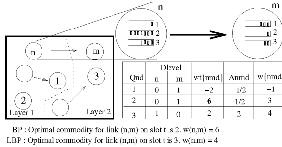
Figure 5.2: An example of the \mathcal{LayBP} execution.
