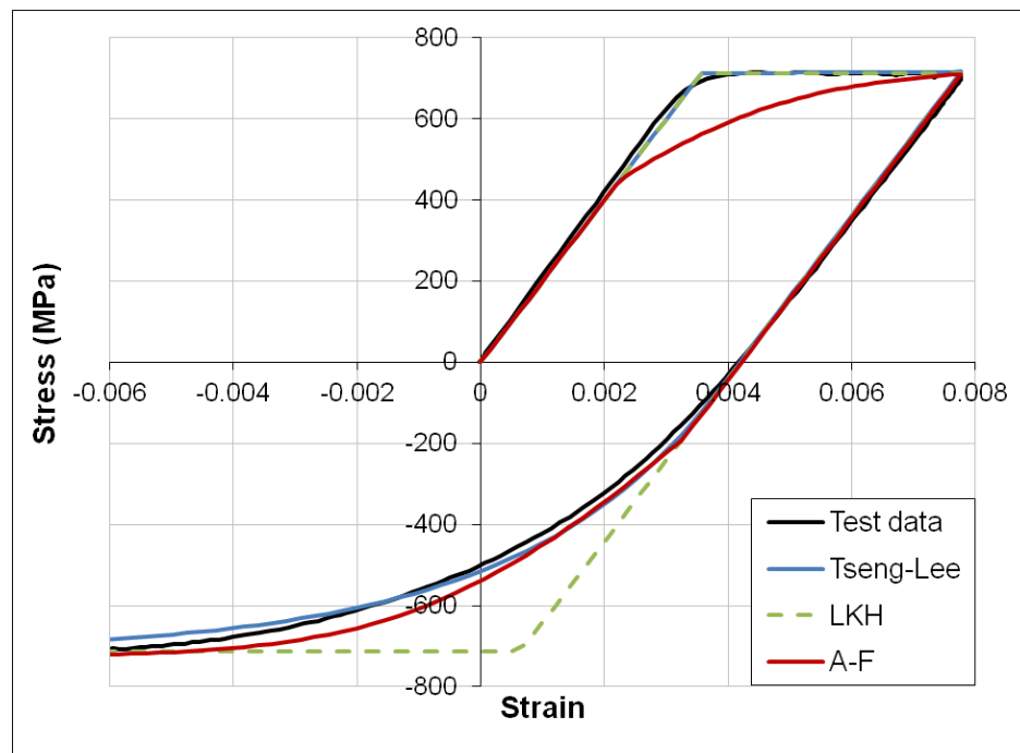
Figure 2.10: Plastic plateau and Bauschinger effect simulation.
