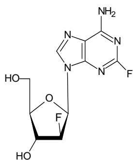
Clofarabine
