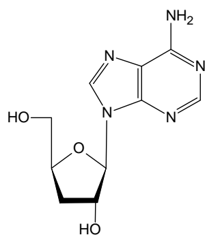
Cordycepin
