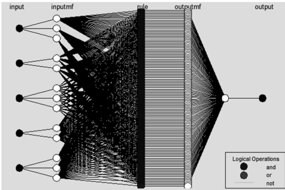
Figure 21. ANFIS 3-2-3-2-3 structure
