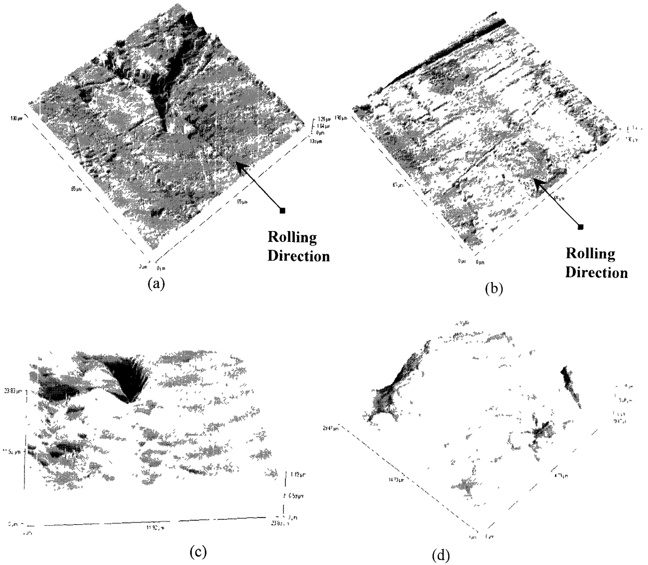
Fig. 4 9: Alloy 2024-T3 (LT plane), 30min in the EXCO solution (a) and (b) different areas (130x130µm), (c) and (d) magnification of previous topographies (30x30µm).
