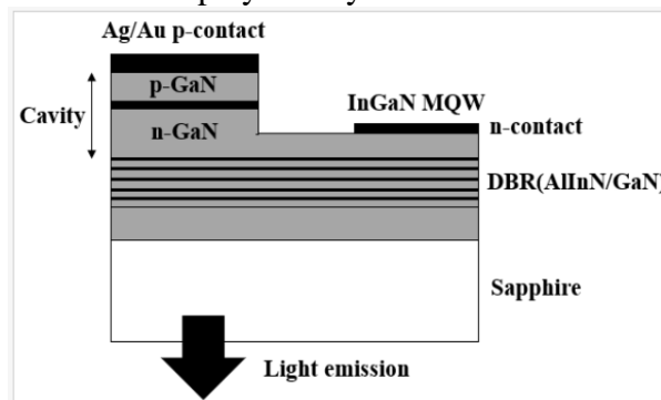
Figure 11. The schematic diagram of a typical rc-LED [57]
