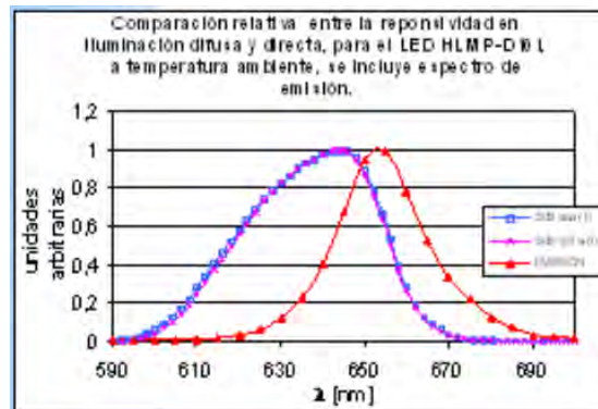
Figure 20. Spectral responsivity of a LED functioning as detector and as emitter [64].
