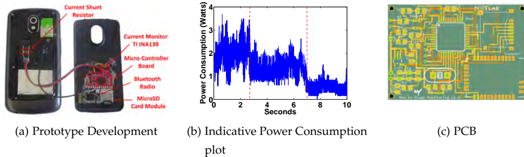
Figure 71: NITOS MMS
