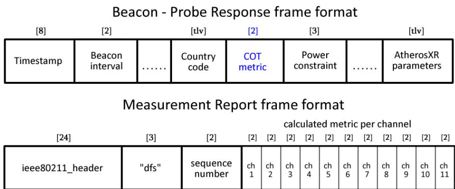
Figure 28: Frame format.
