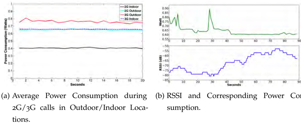
Figure 73: Experimental Results.
